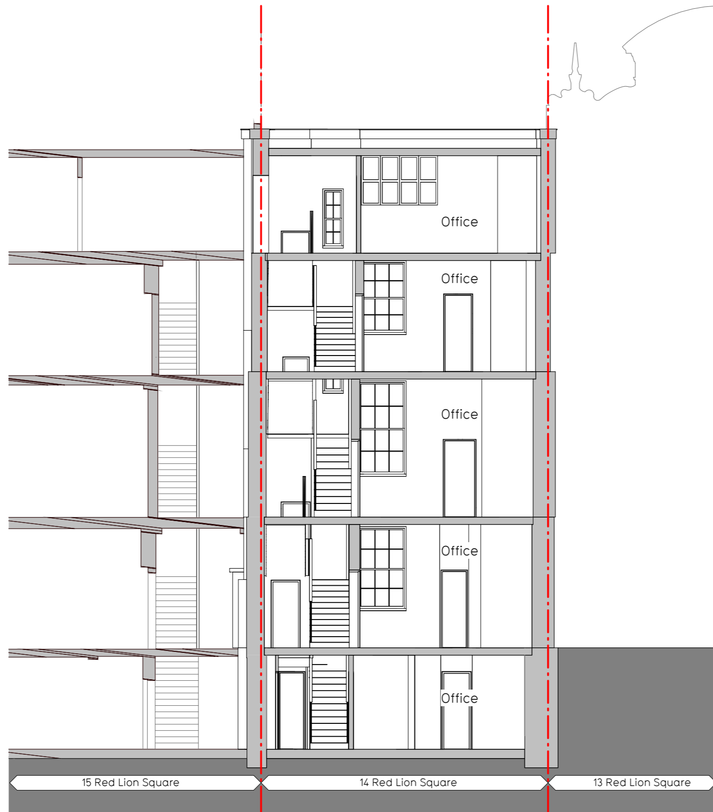
B Existing - Section BB 021 1:100
