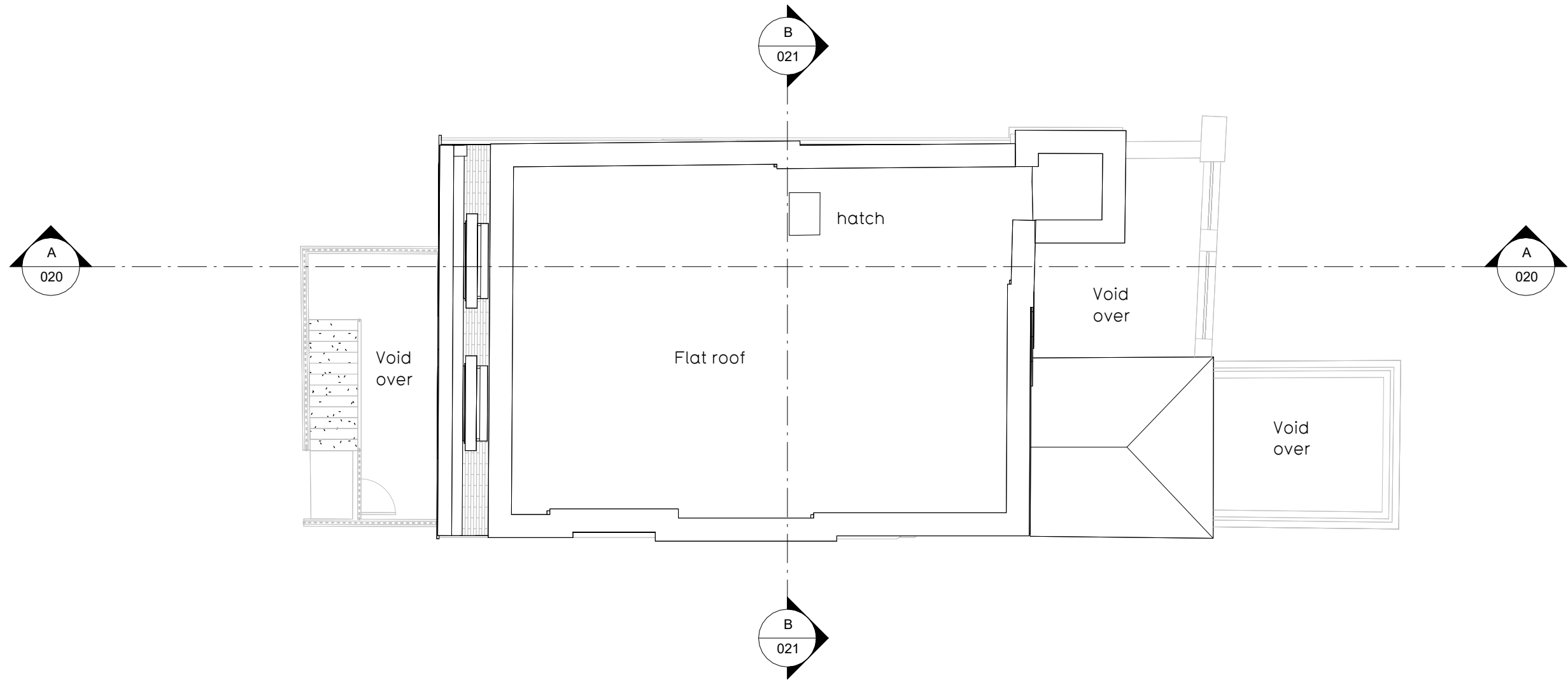
1 Existing - Roof Plan 015 1 : 100
