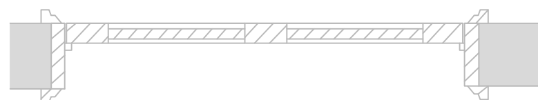
SIMPLE 6 PANEL DOOR DETAIL PLAN
