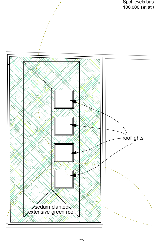
Roof Plan
