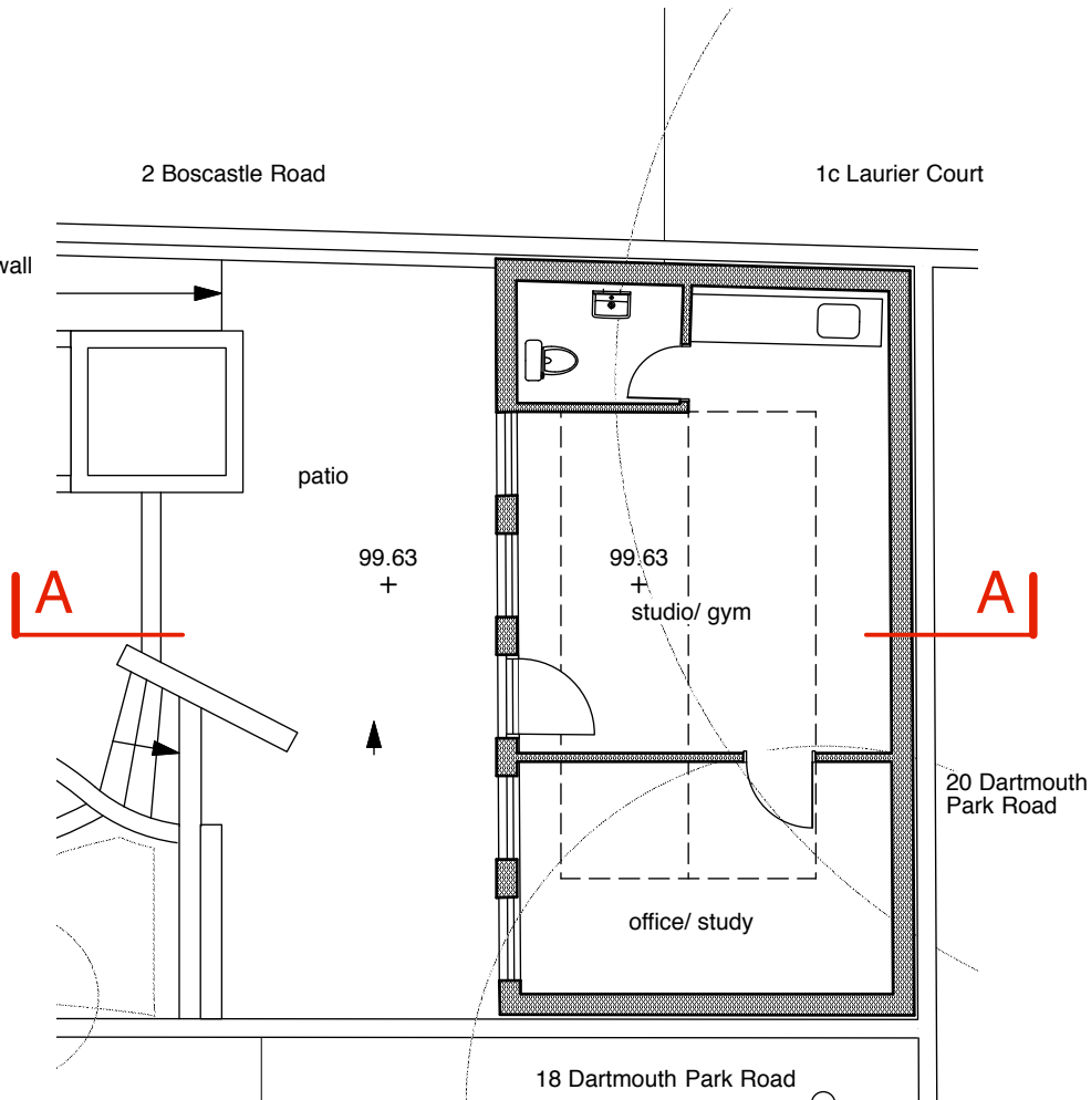
Ground Plan
