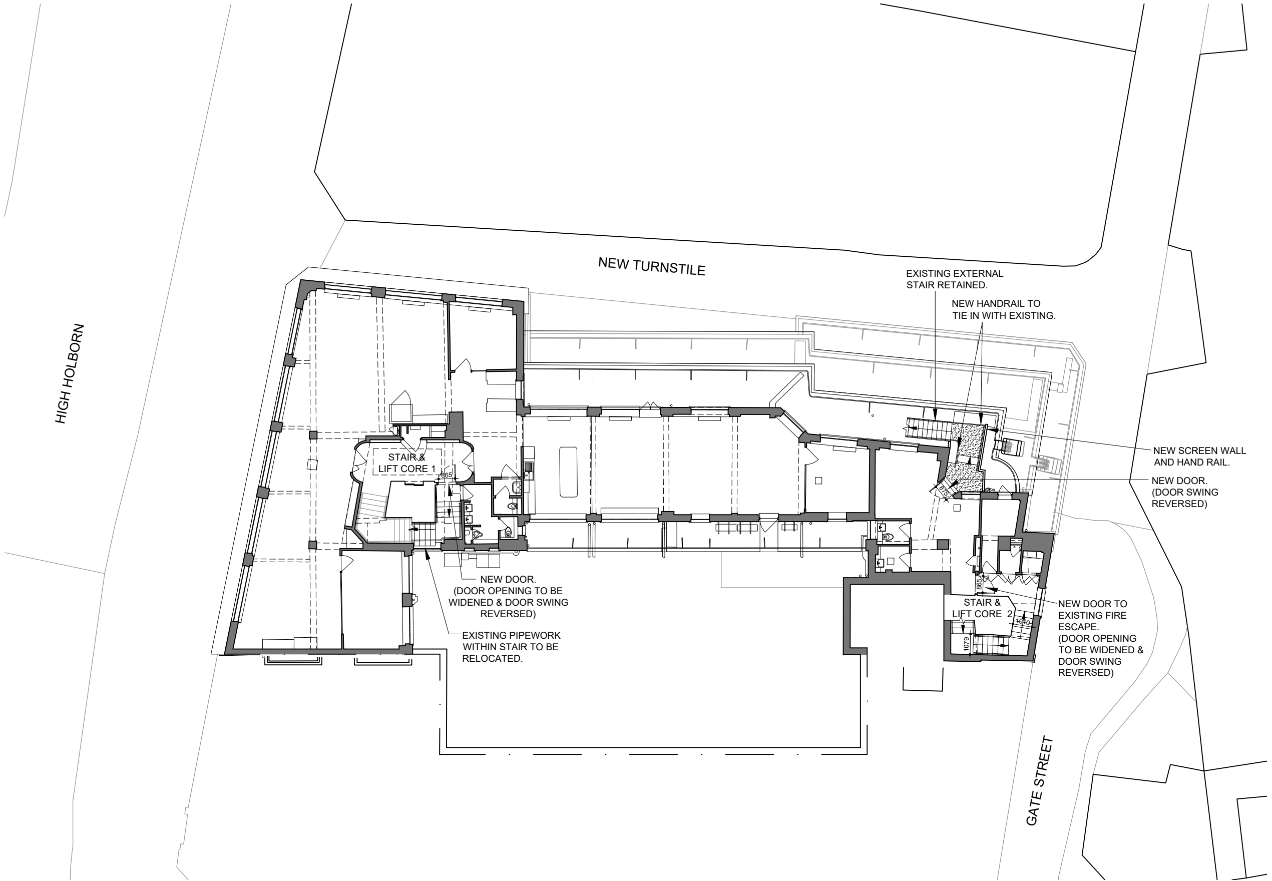
LEVEL 7 - PROPOSED SEVENTH FLOOR PLAN
