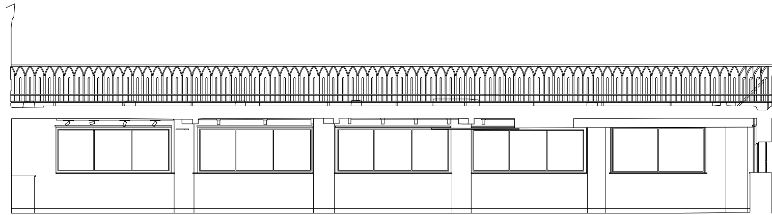
SECTIONAL ELEVATION 1
