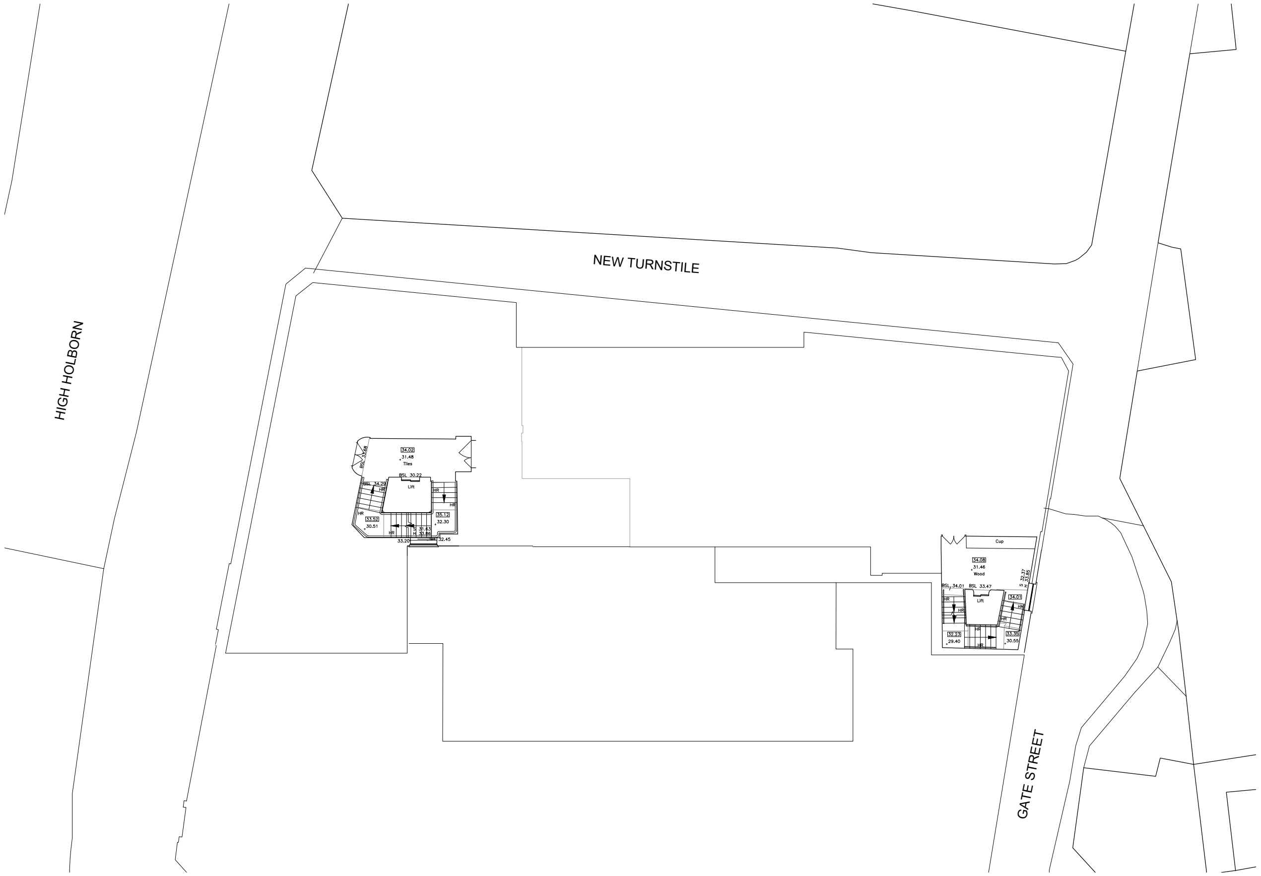
LEVEL 2 - SECOND FLOOR PLAN
