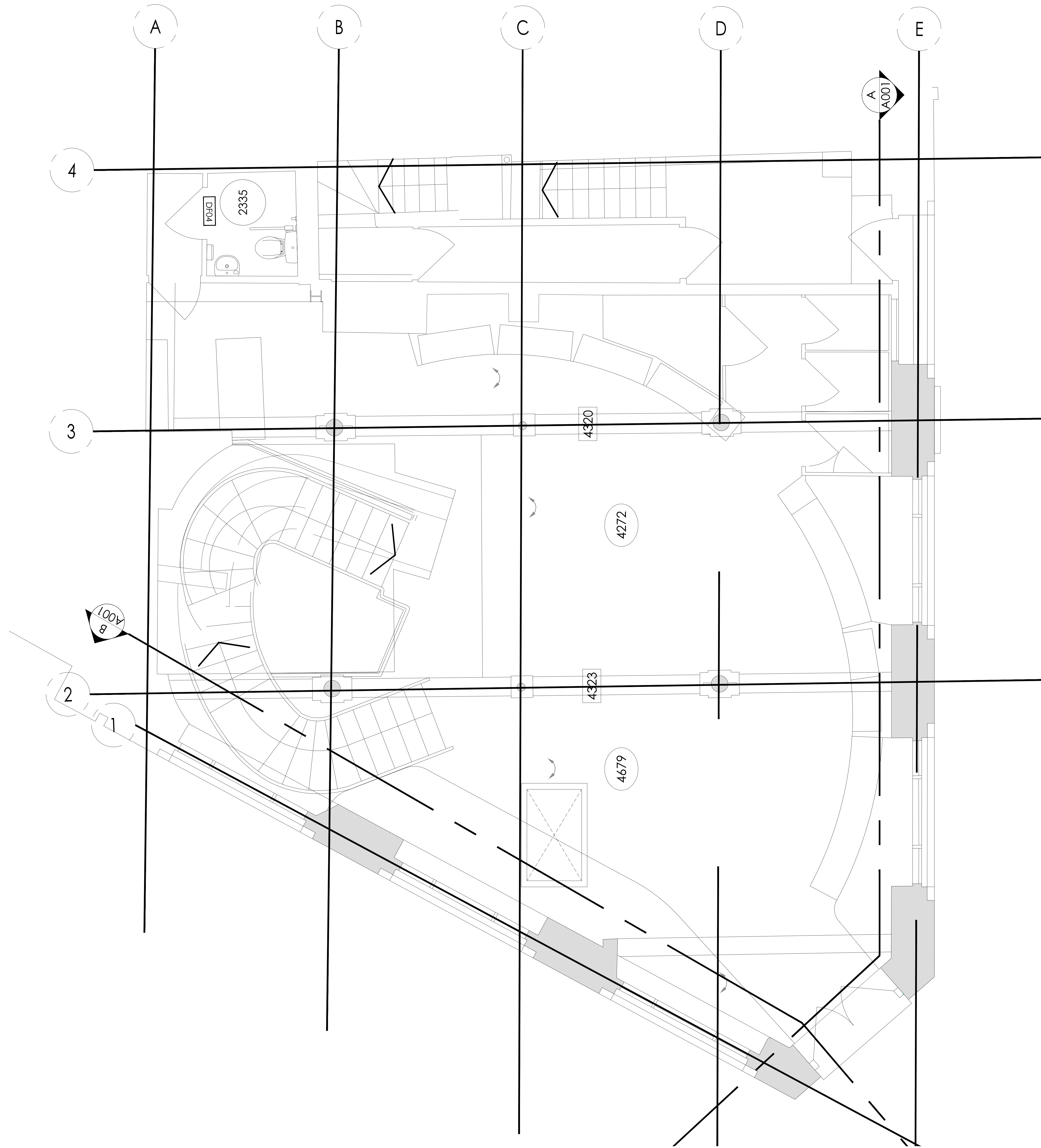
2 EXISTING - GROUND FLOOR SCALE: 1:25
