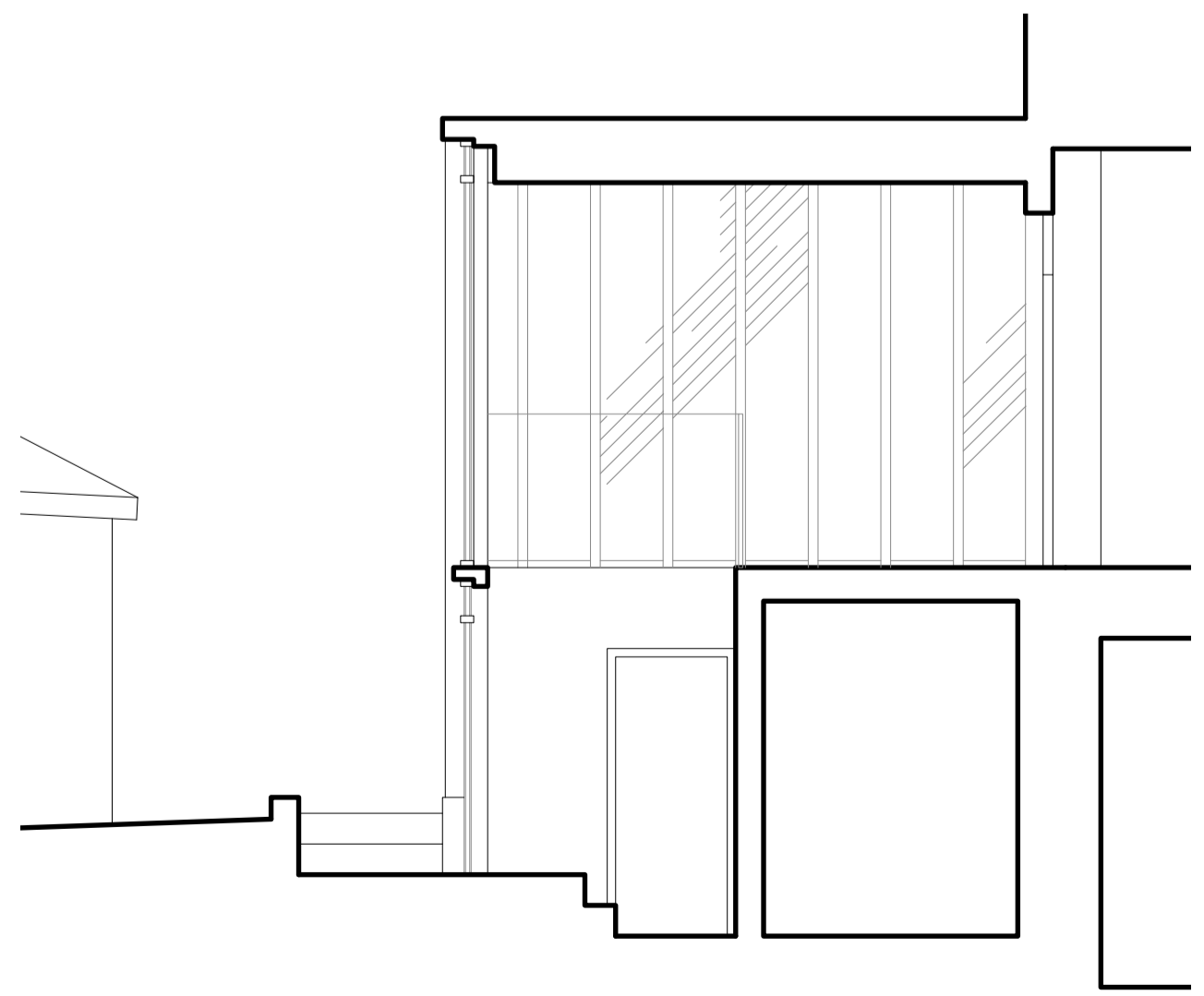
Proposed Section D-D
