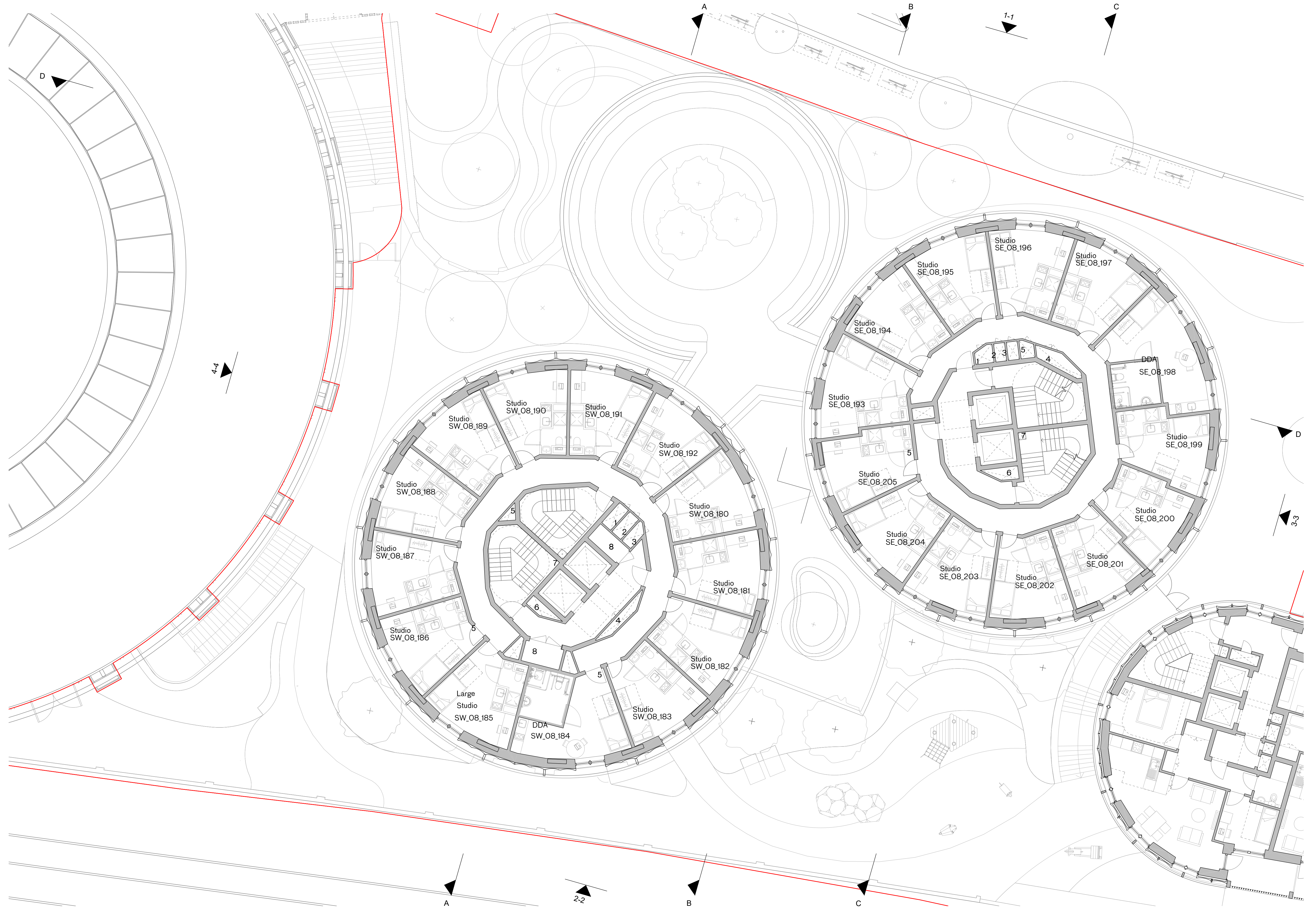
PBSA Building - Proposed Eighth Floor Plan
