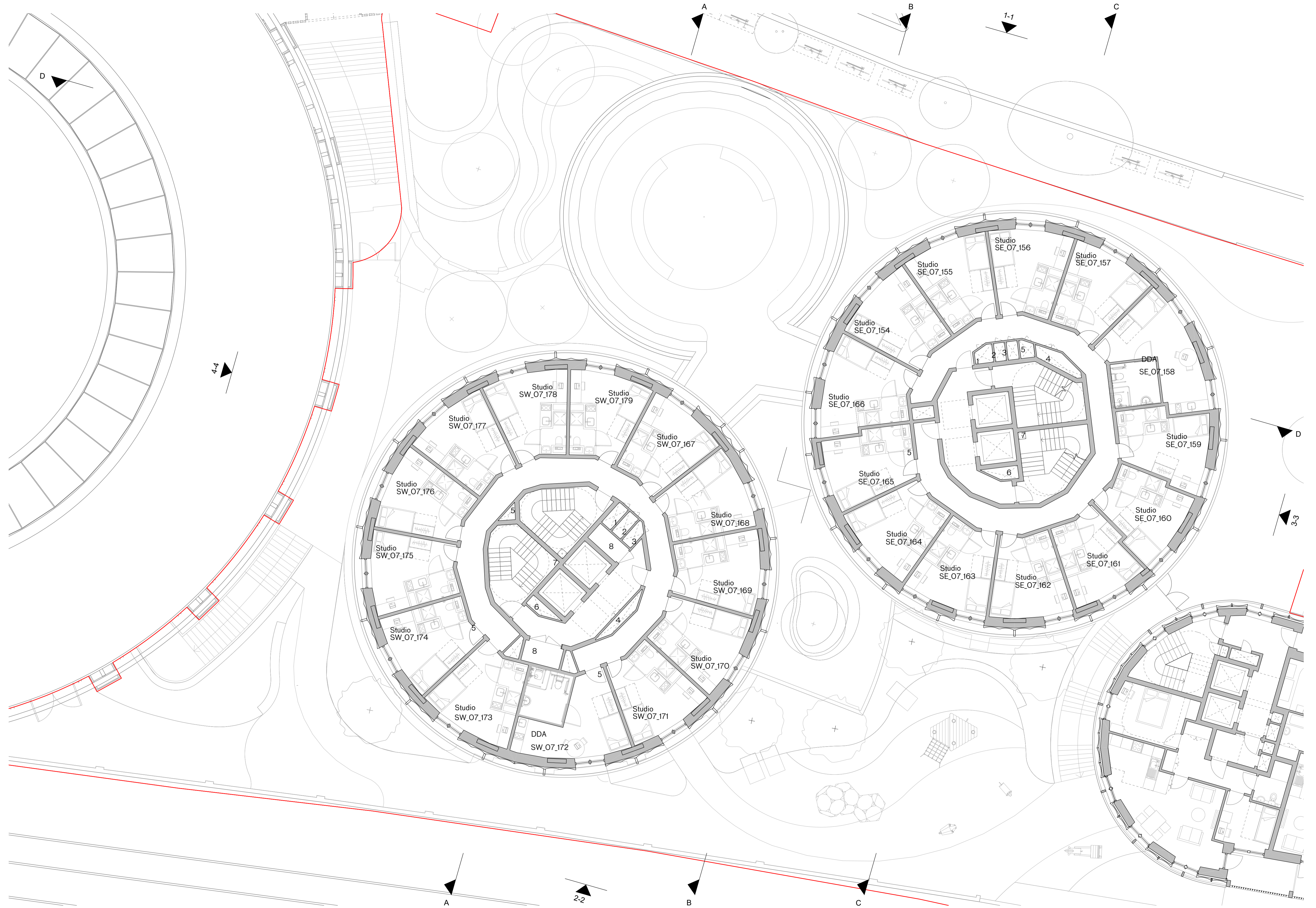
PBSA Building - Proposed Seventh Floor Plan
