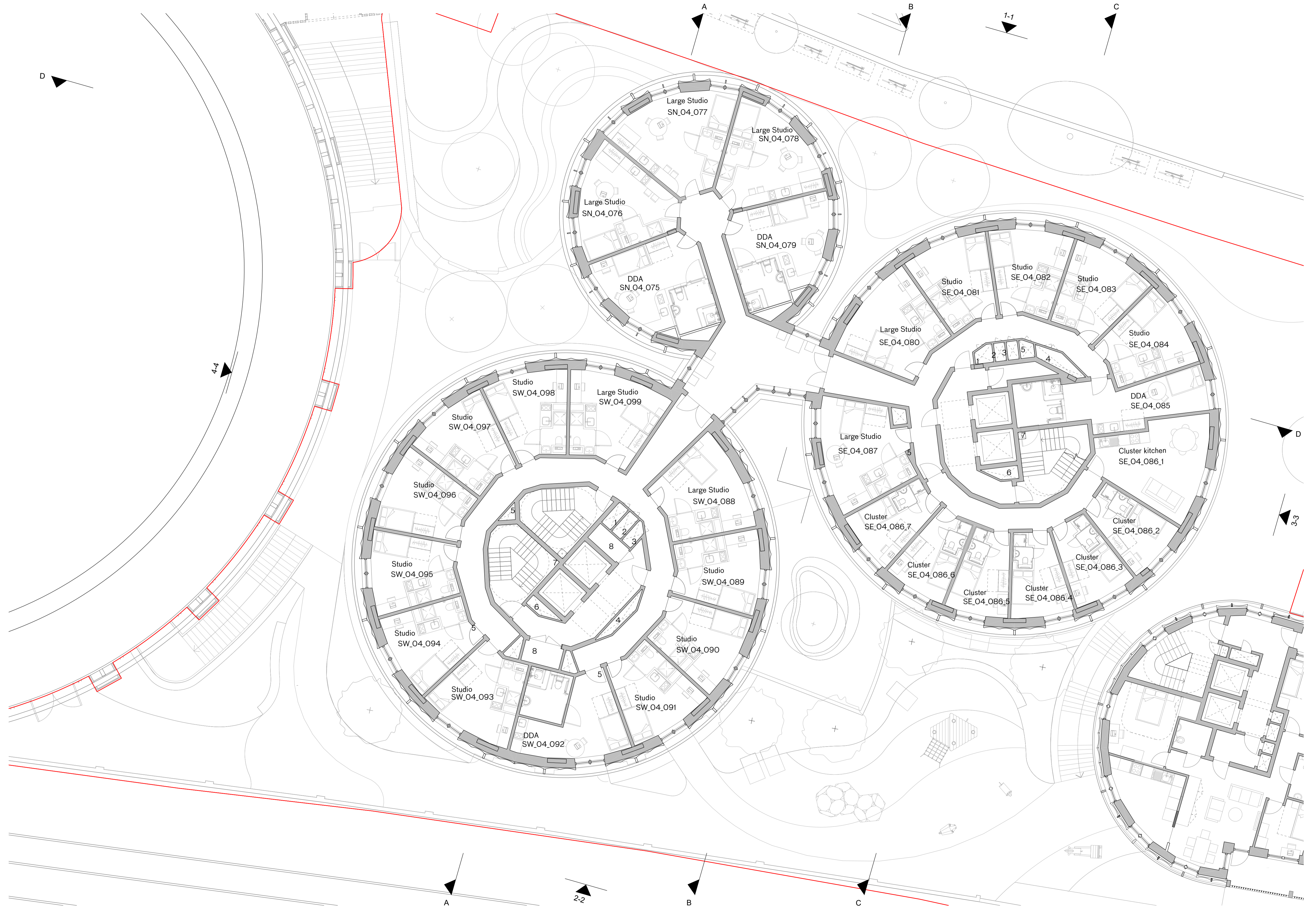
PBSA Building - Proposed Fourth Floor Plan
