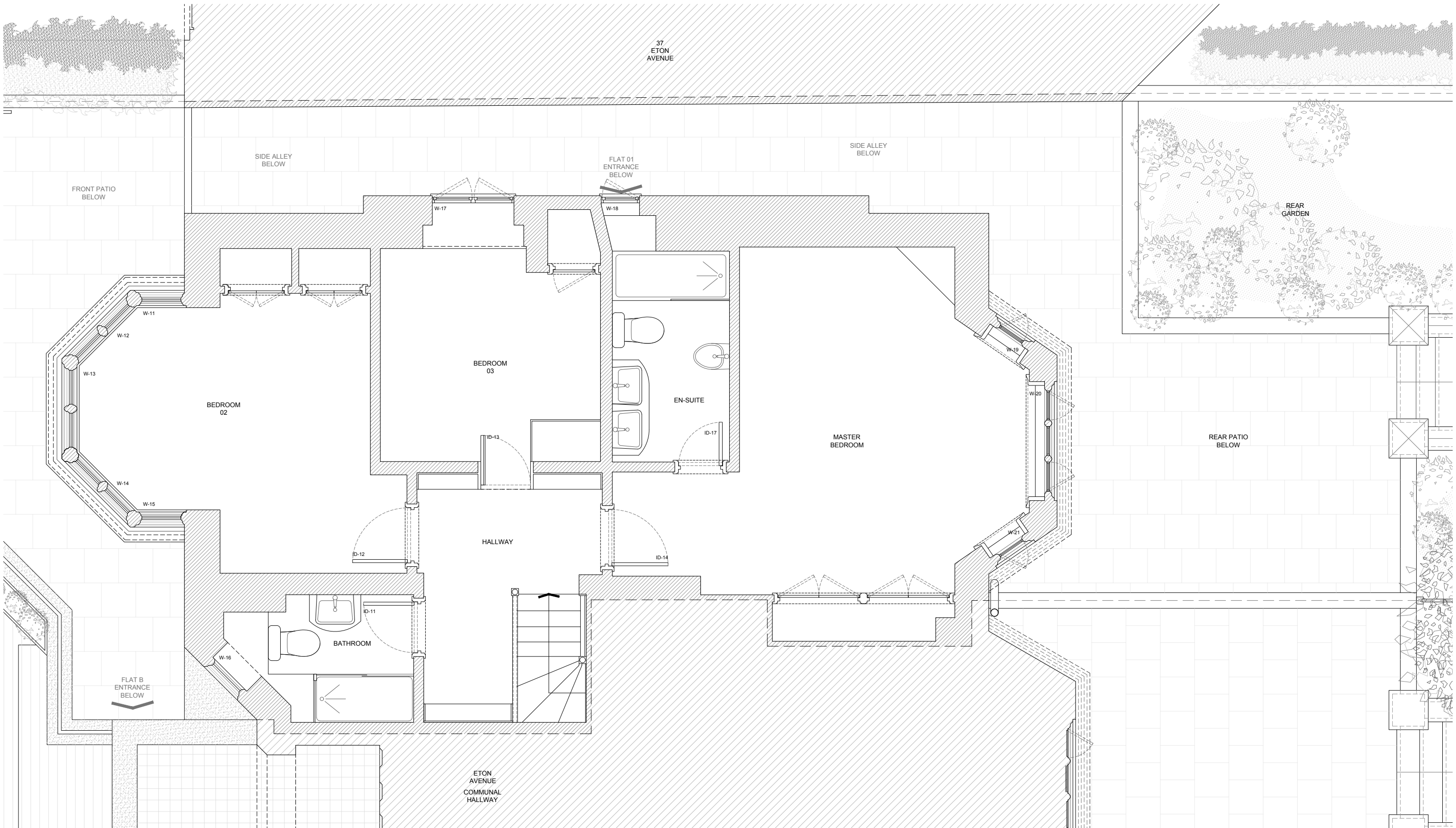
ENLARGED UPPER GROUND FLOOR PLAN 1:50 / A3
