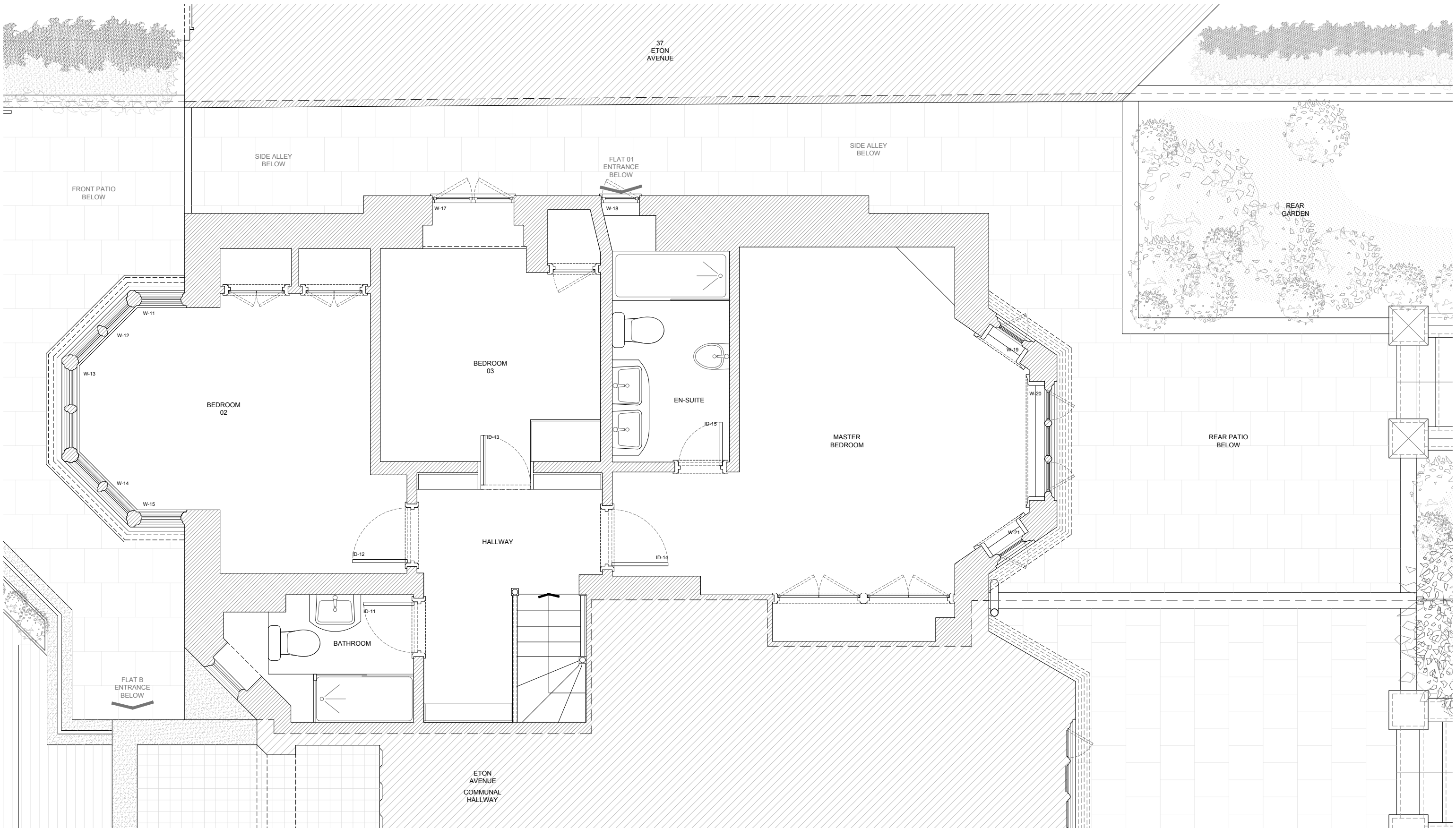
DEMOLITION UPPER GROUND FLOOR PLAN 1:50 / A3
