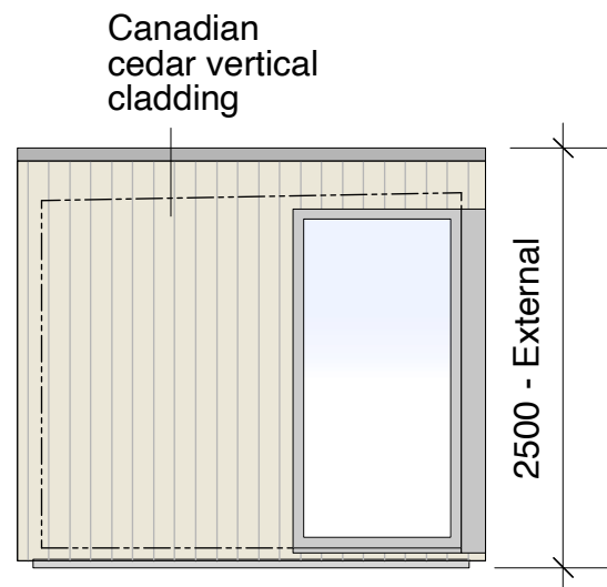
Left elevation
