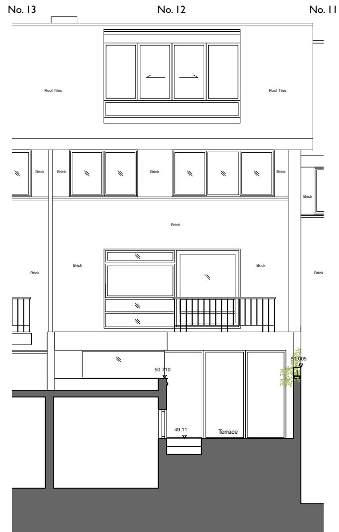
00 - Existing Rear Section/Elevation 1:100@A3
