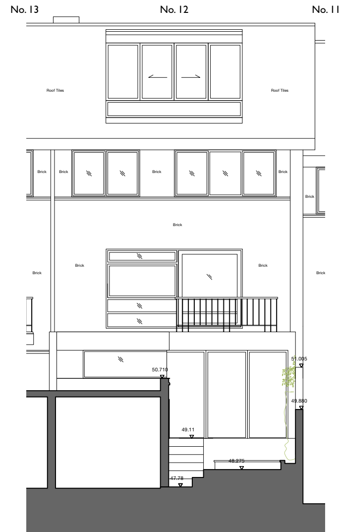
01 - Existing Rear Section/Elevation 1:100@A3
