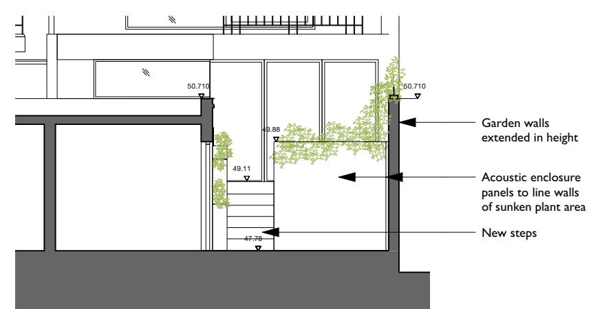
03 - Approved Rear Section/Elevation 1:100@A3
