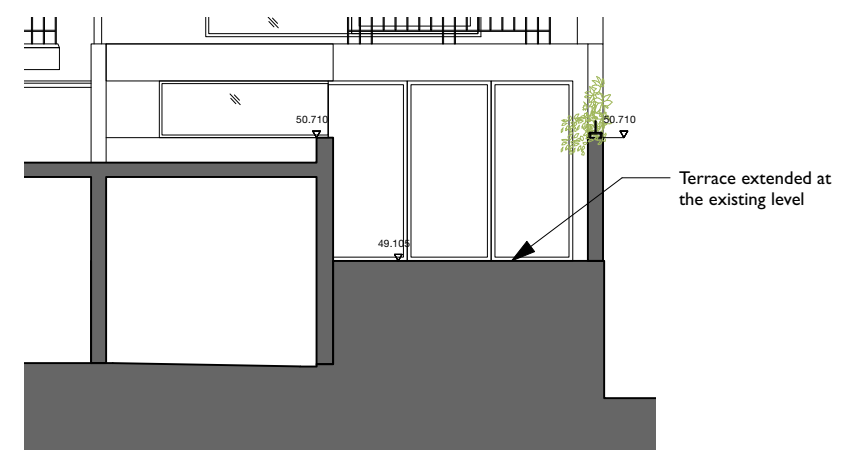
02 - Approved/Proposed Rear Section/Elevation 1:100@A3
