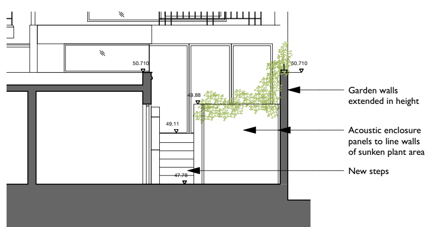
04 - Proposed Rear Section/Elevation 1:100@A3
