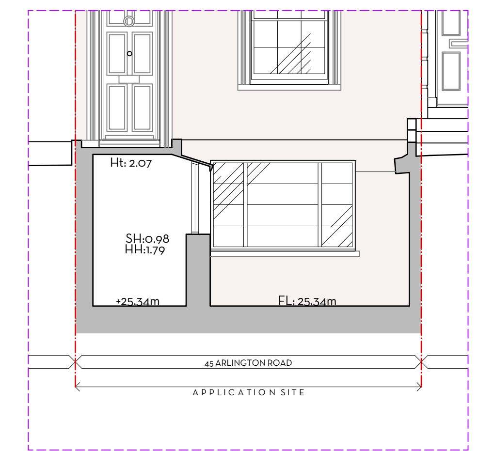
Section through Lightwell
