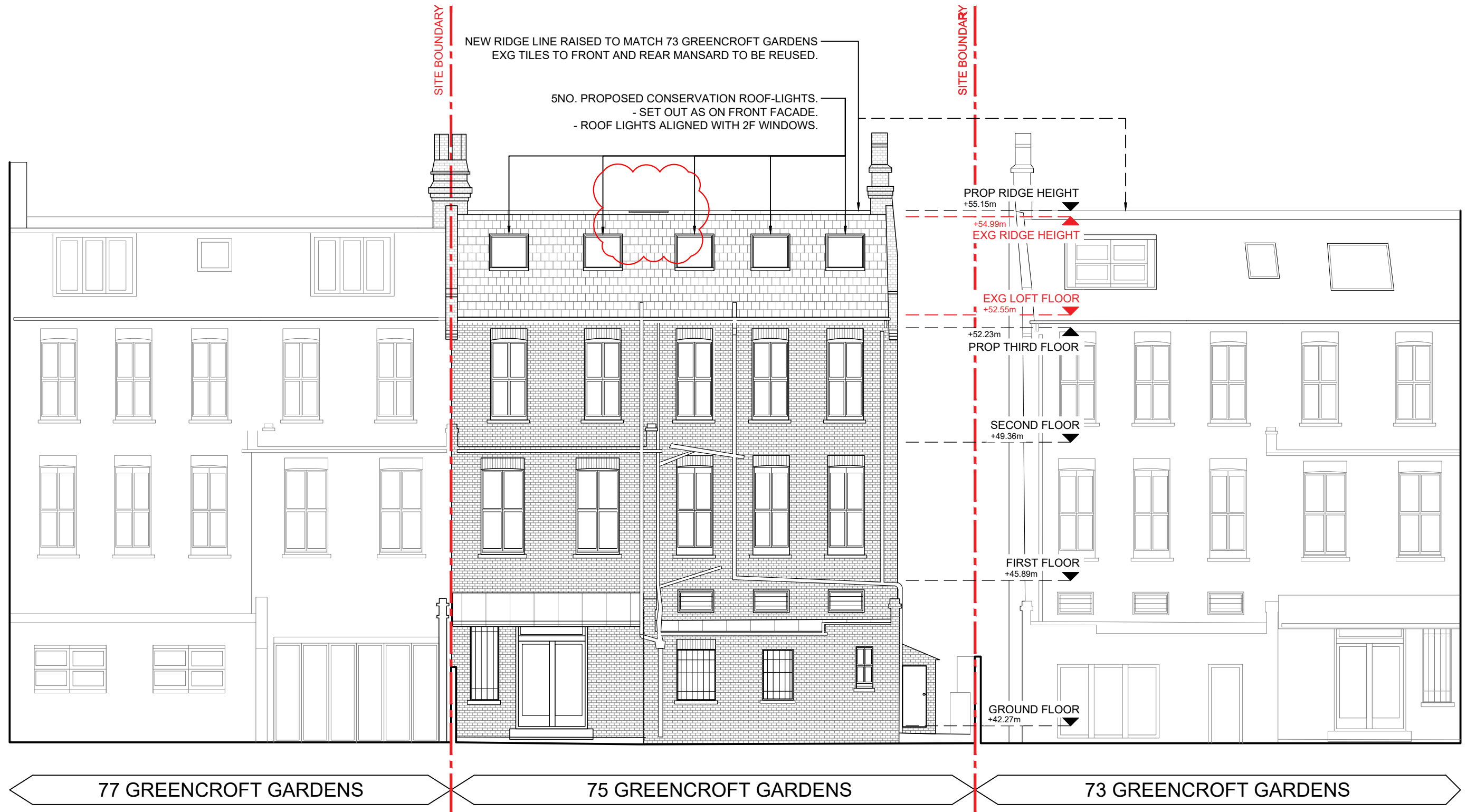
01 PROPOSED - REAR ELEVATION SCALE // 1:100
