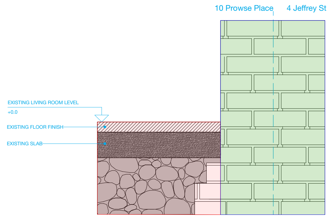
1 Existing Floor Build Up 1:10
