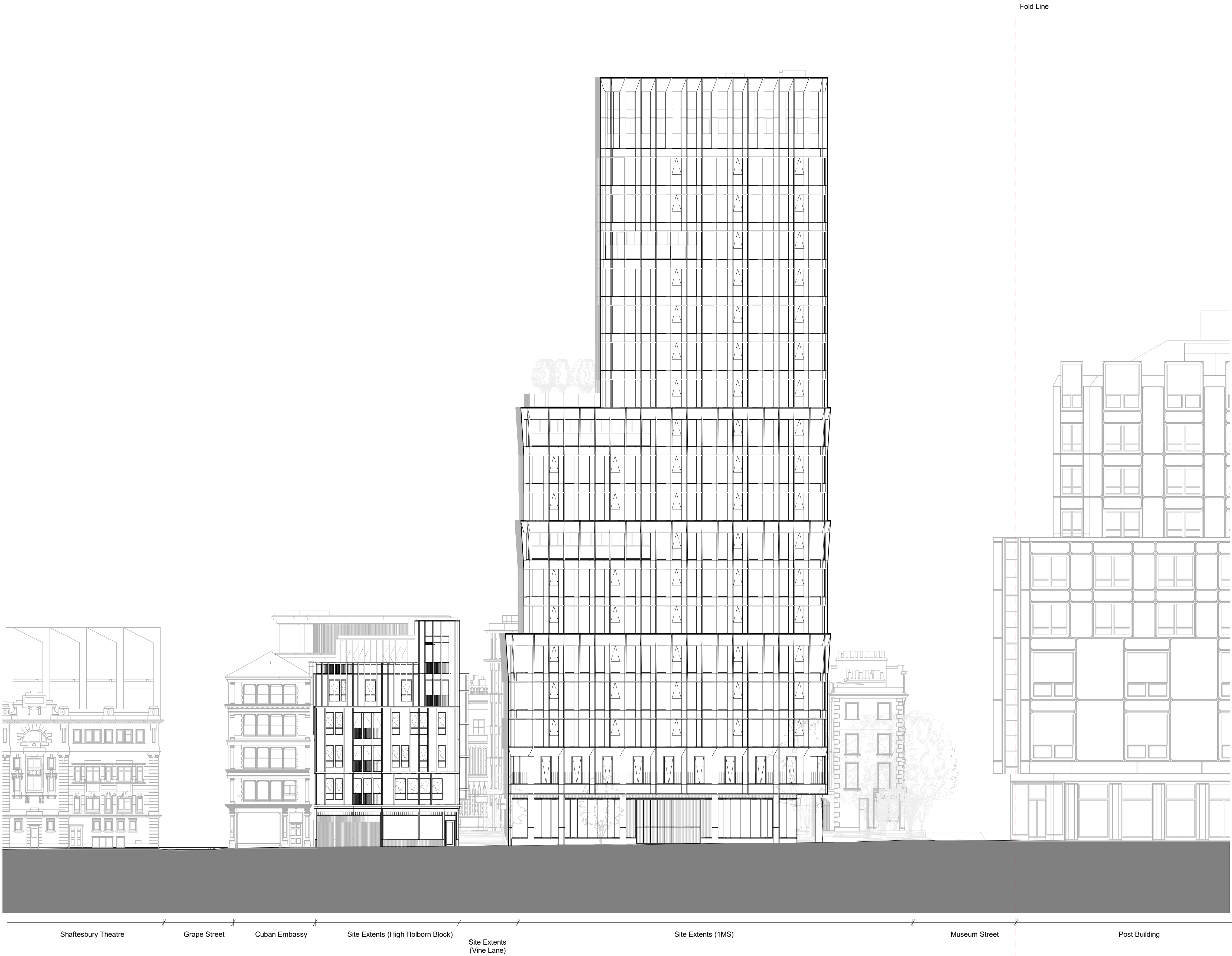
2 Proposed High Holborn Elevation
