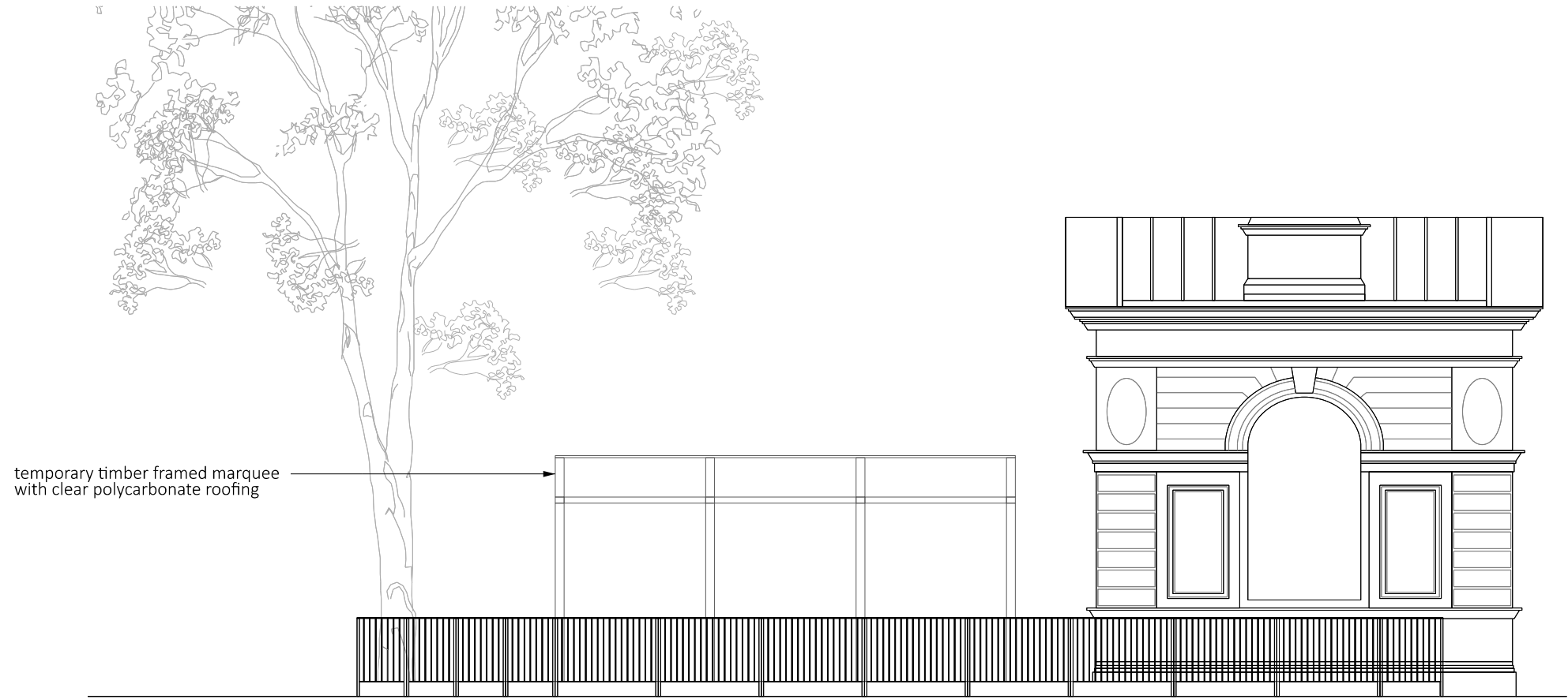
01 Proposed South West Elevation
