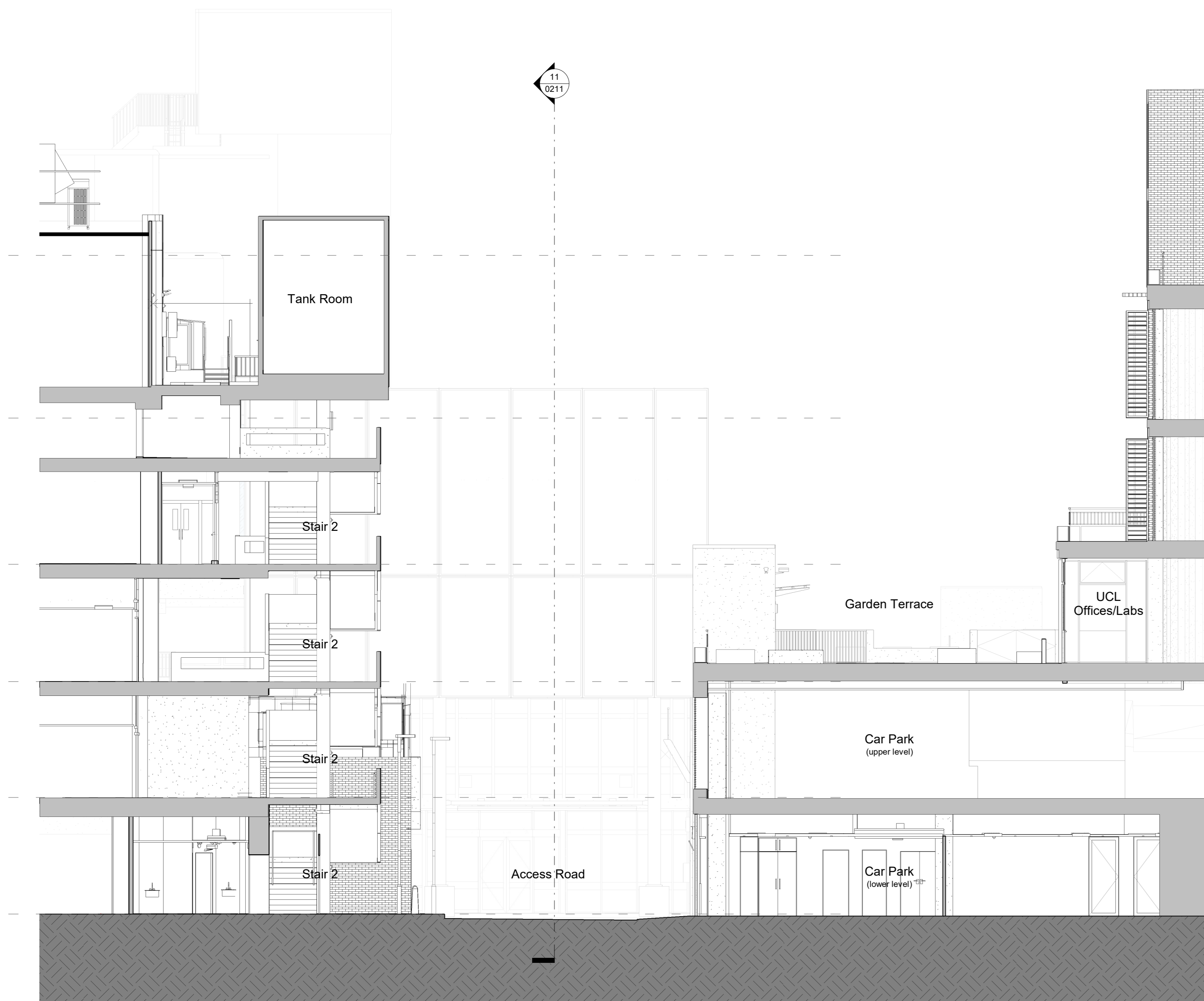
1 EXISTING - Section 01 - Cross-Section Through Stair 2 1 : 100
