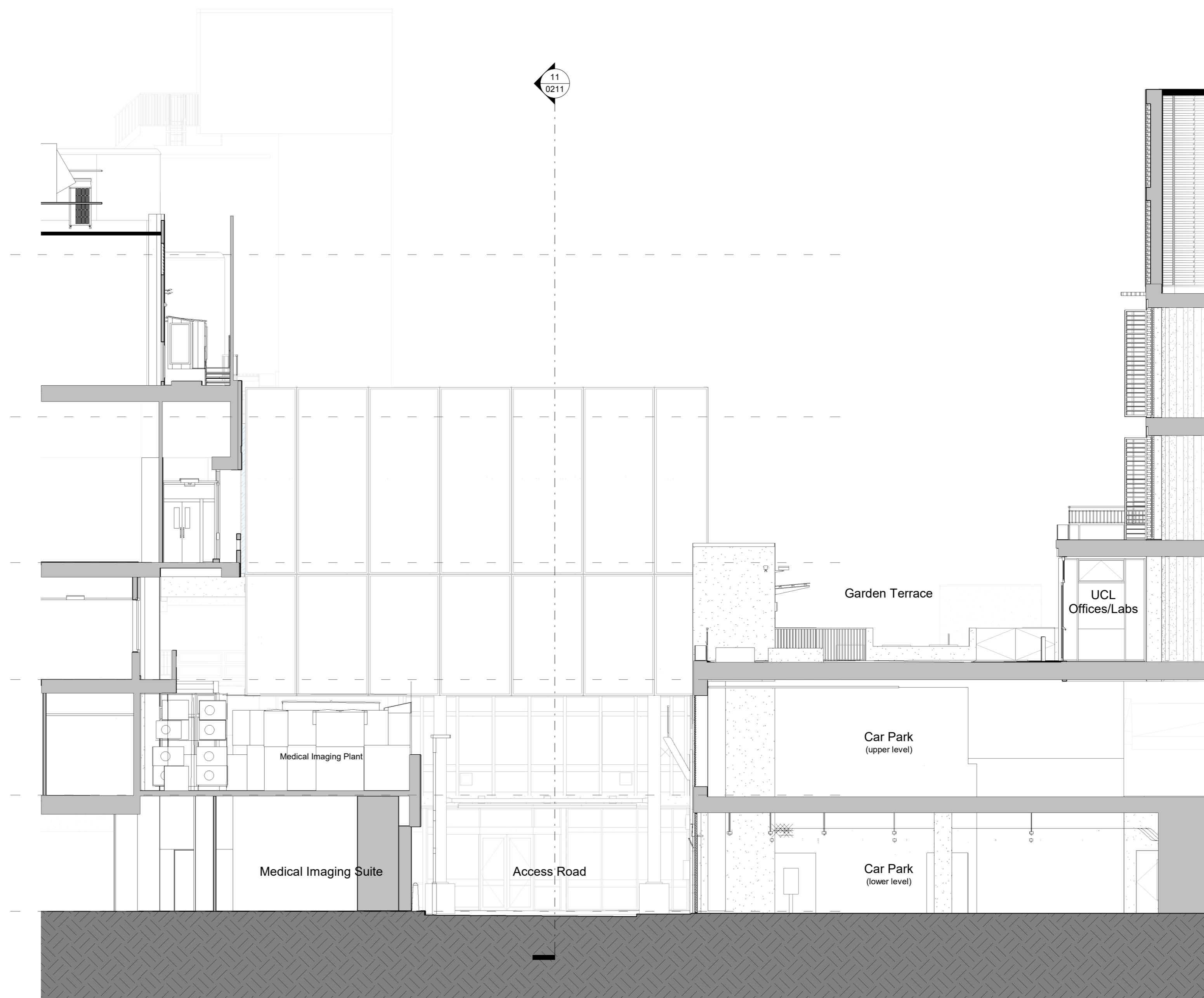
2 EXISTING - Section 02 - Cross-Section Through MRI Suite 1 : 100
