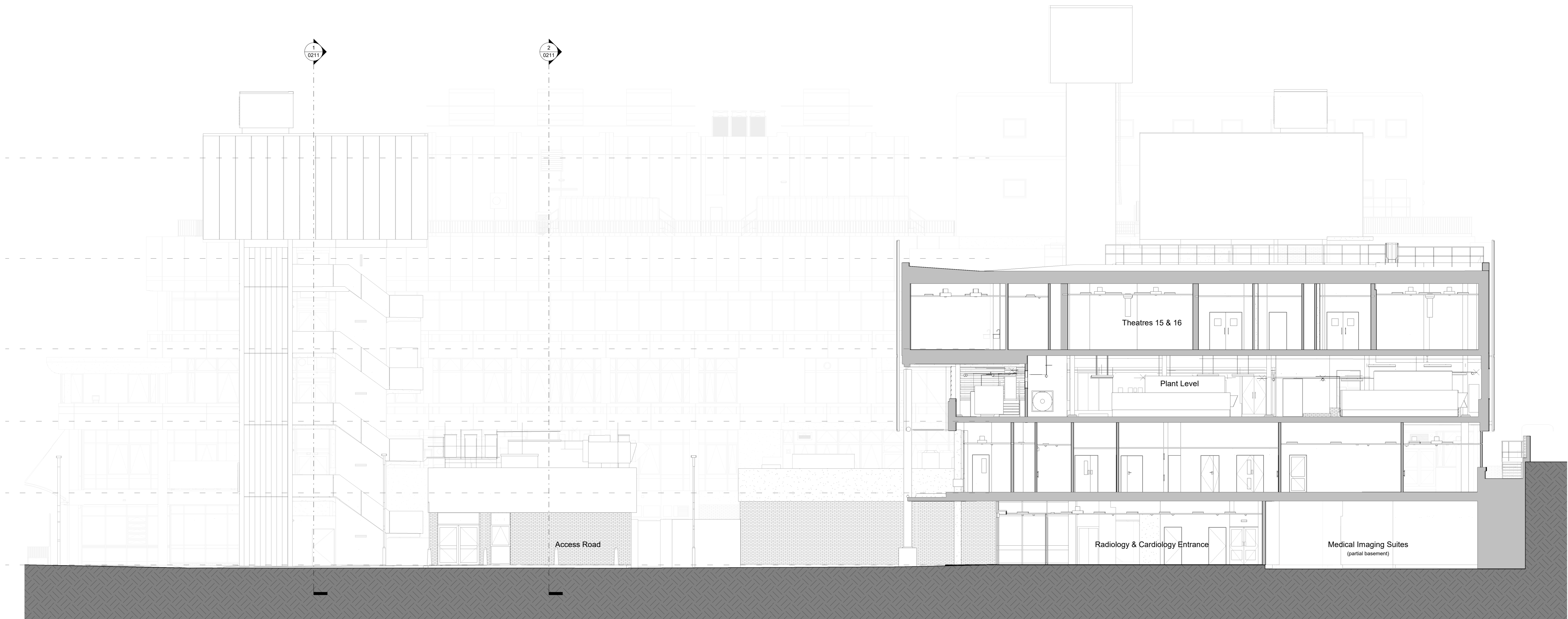
11 EXISTING - Section 11 - Long Section Through Access Road 1 : 100
