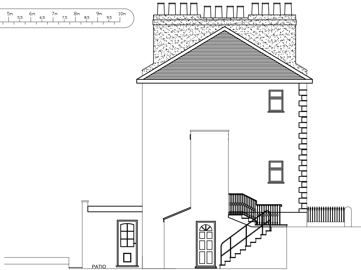
SIDE ELEVATION EXISTING (AS VIEWED FROM NO:3)
