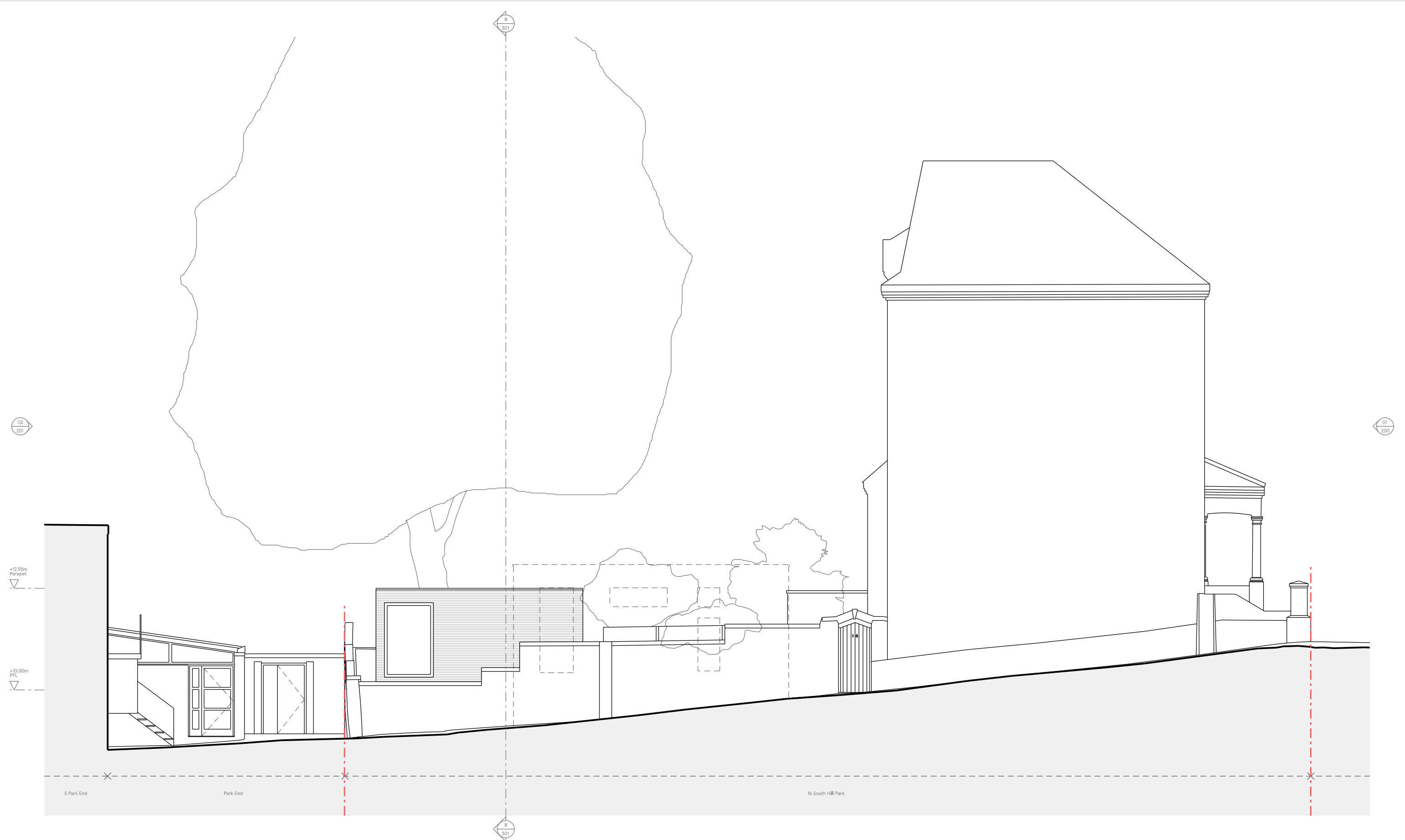
01 South Elevation
