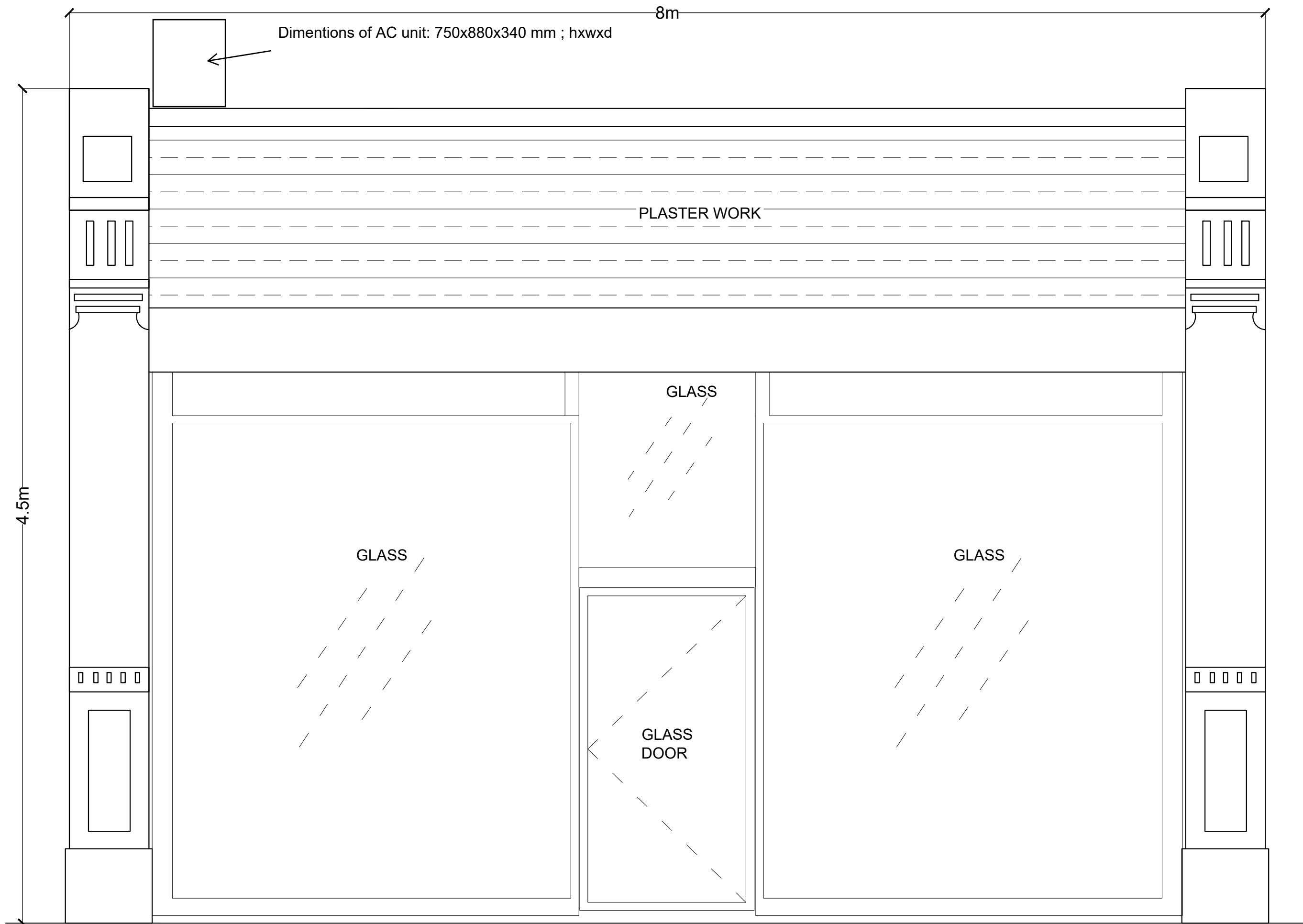
PROPOSED CAFE ELEVATION(AC INSTALLATION) SCALE 1:100 @ A3
