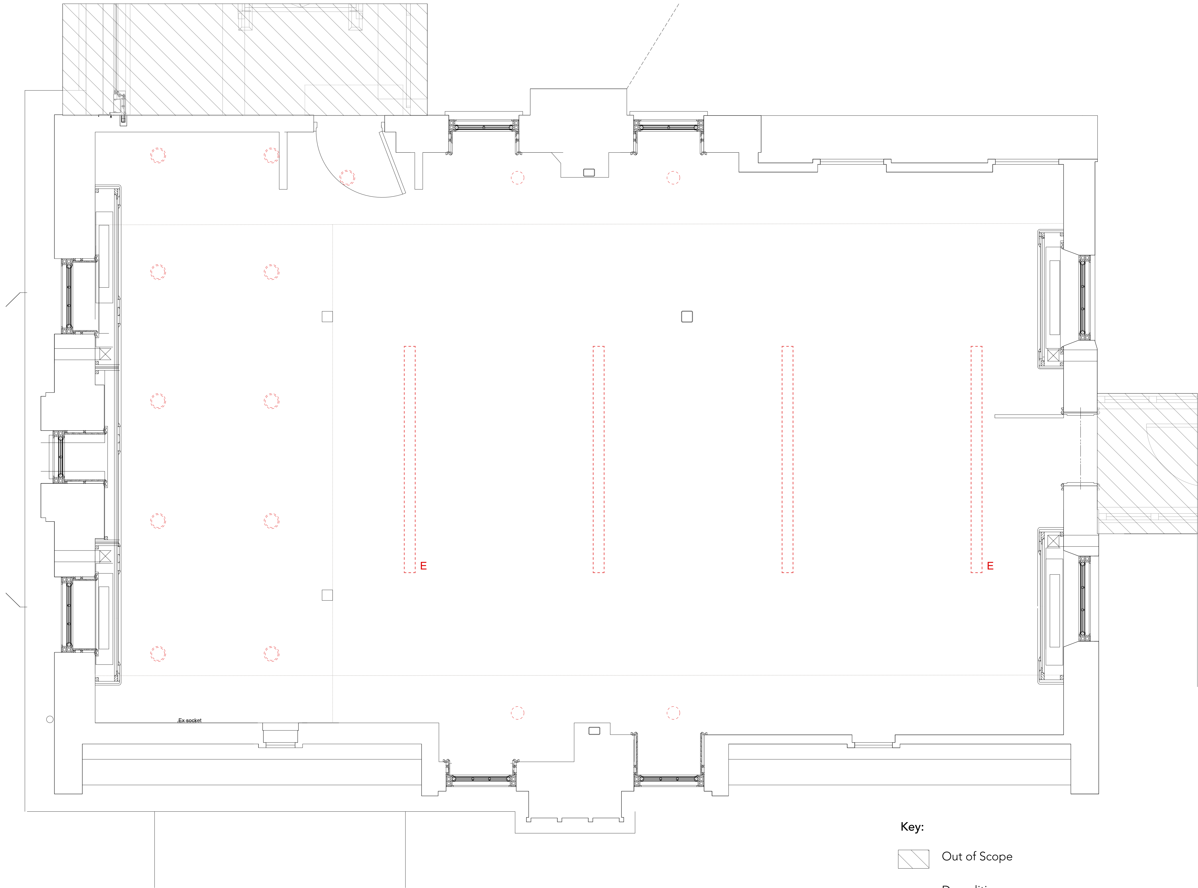
1 Ceiling Demolition Plan Scale: 1:25
