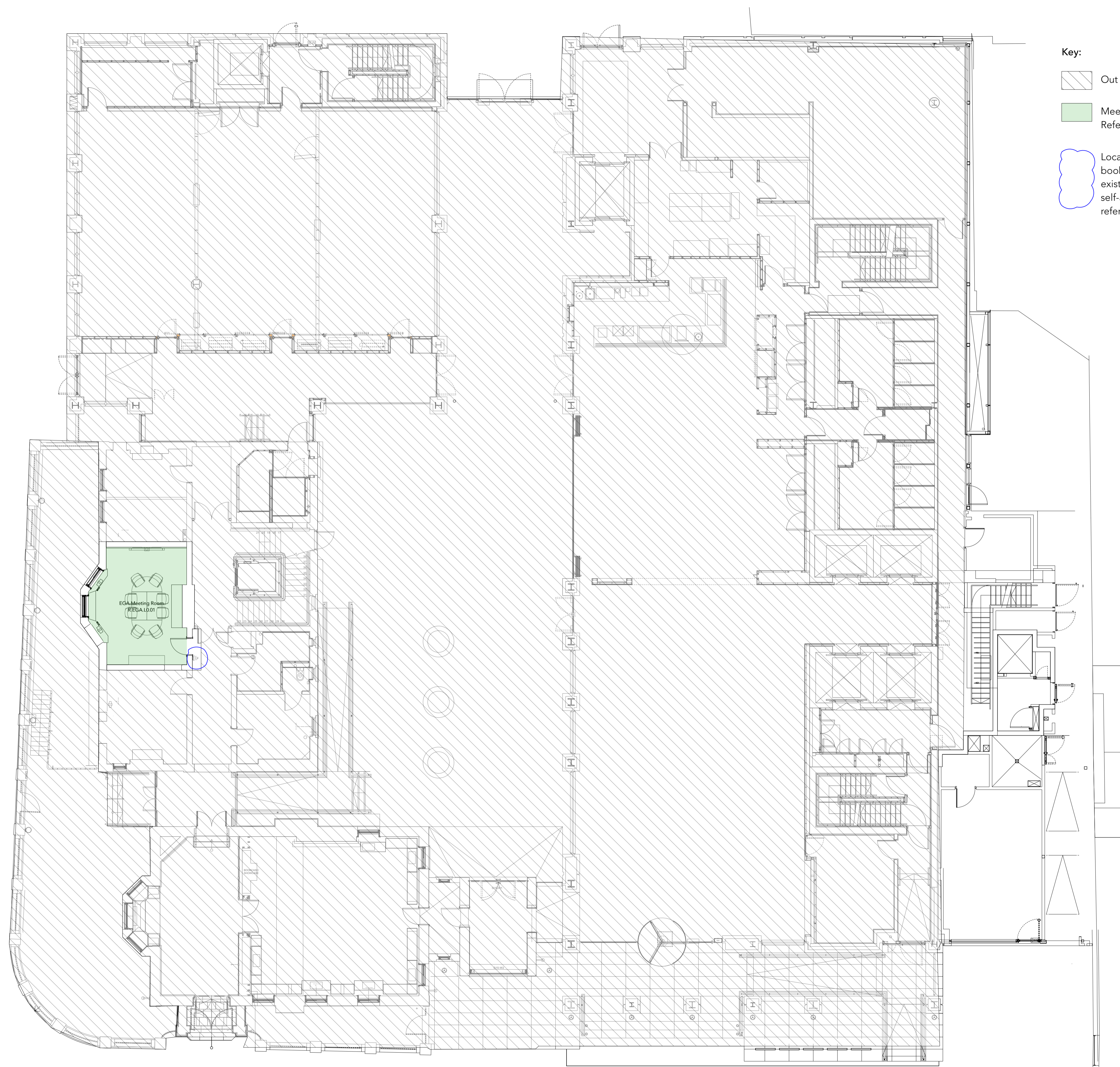
1 Ground Floor Plan Scale: 1:100
