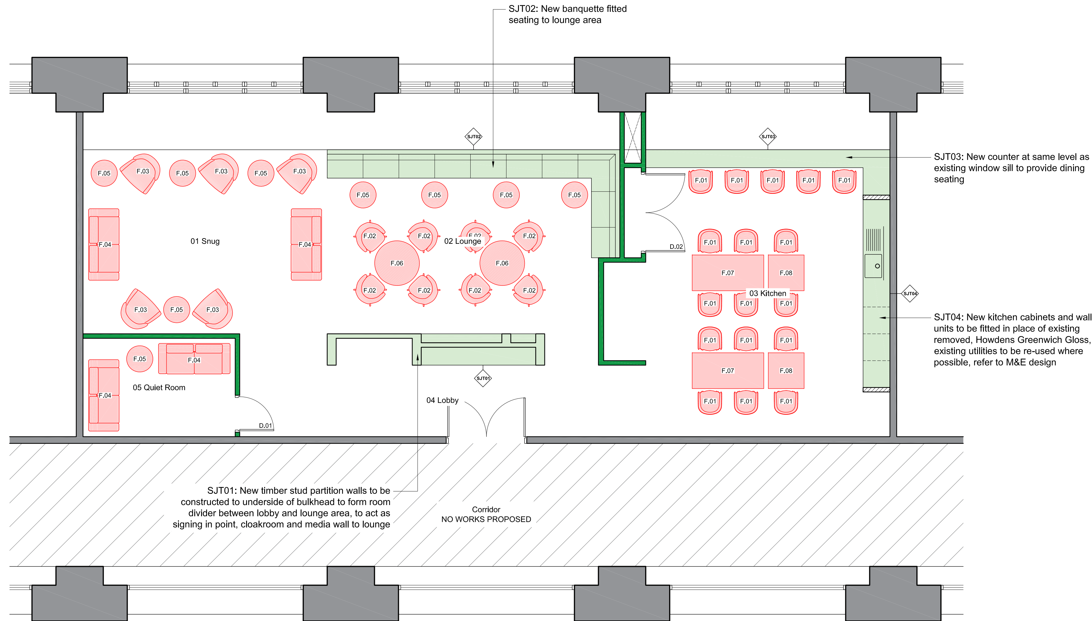
01 Proposed GA Plan Scale 1:50 @ A1
