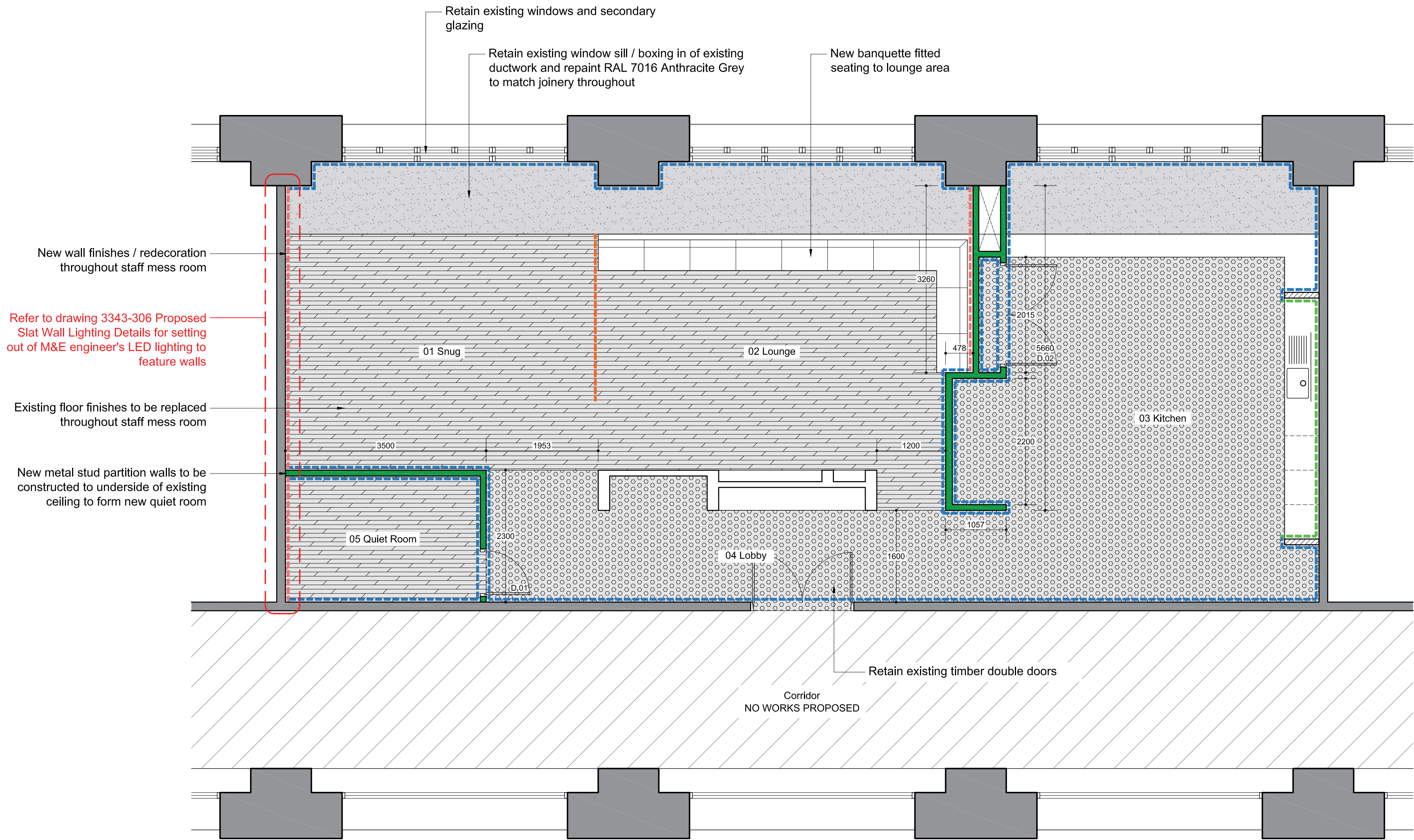
01 Proposed GA Plan Scale 1:50 @ A1
