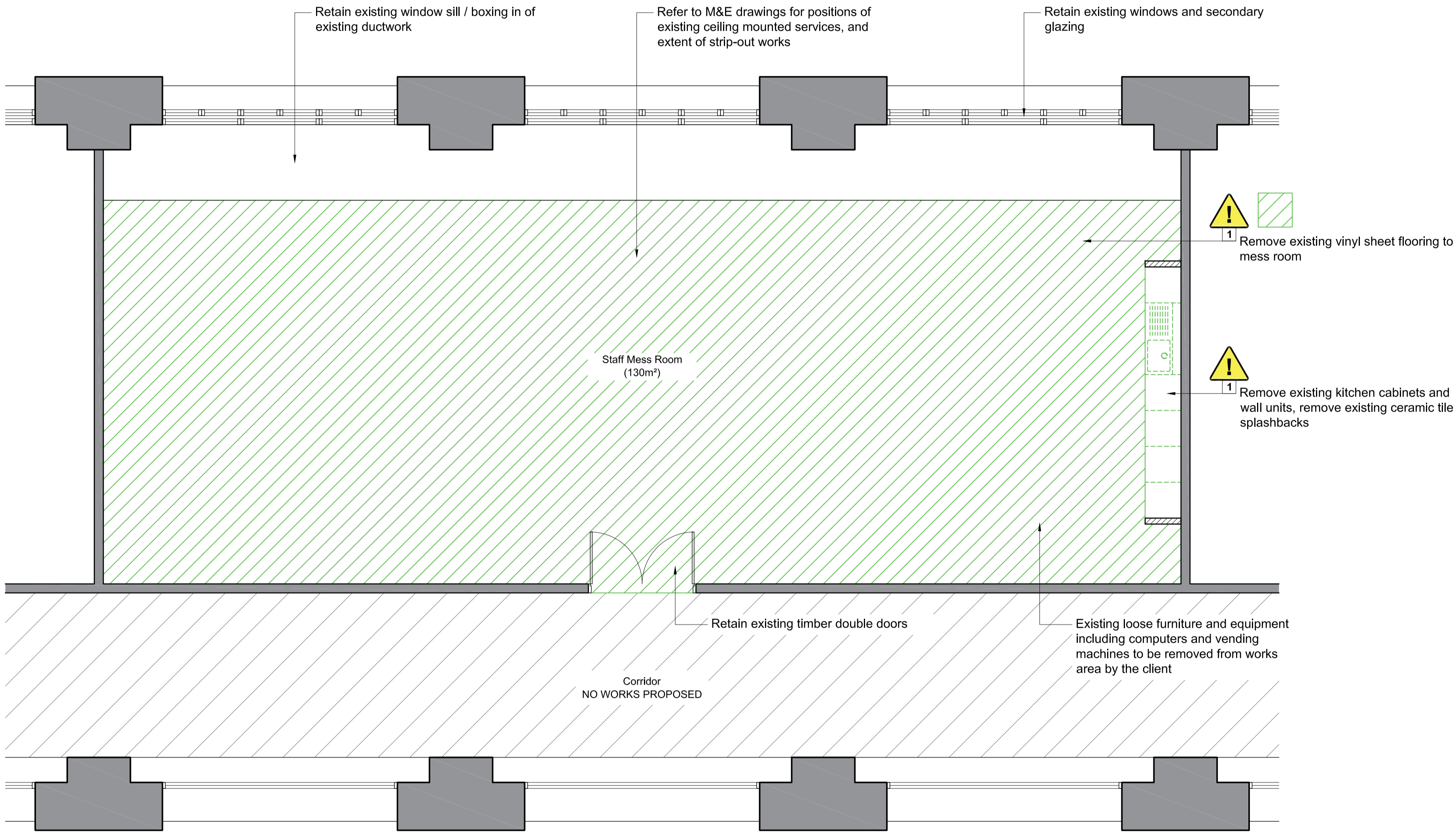
01 Proposed Demolition and Alterations Plan Scale 1:50 @ A1
