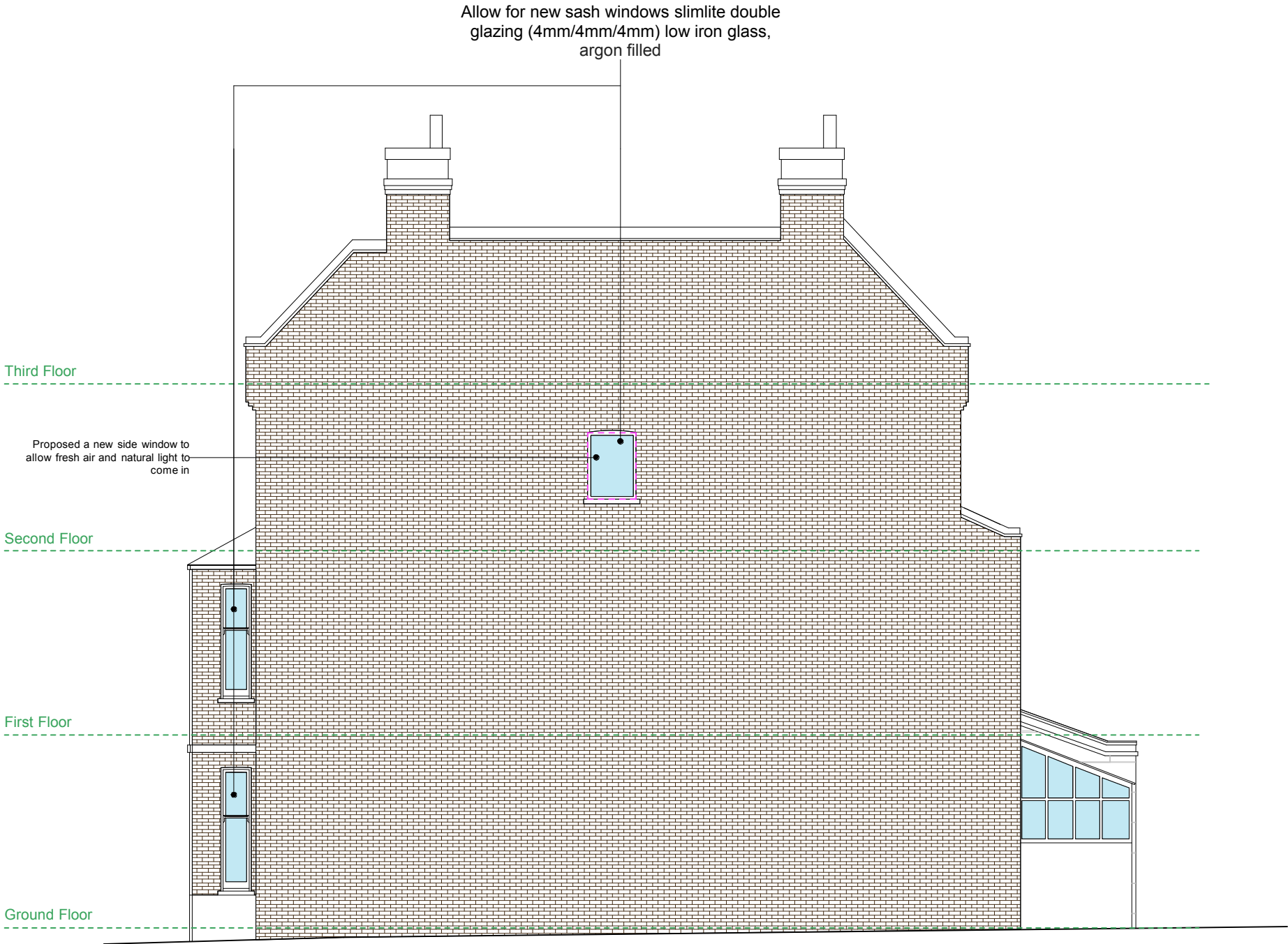
10 NORTH WEST ELEVATION Scale: 1:100
