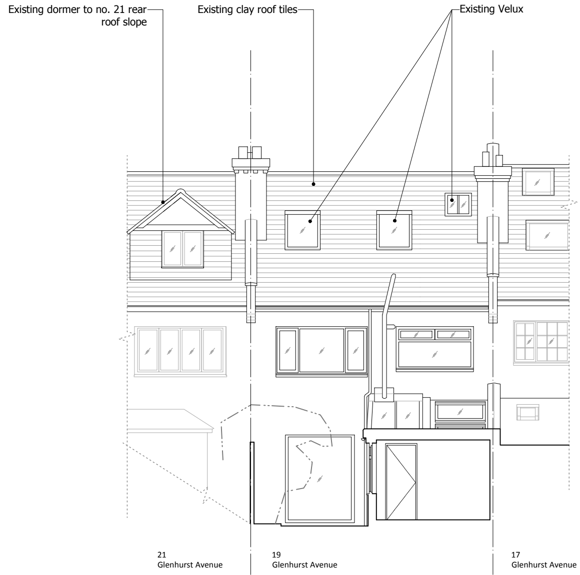
REAR ELEVATION
