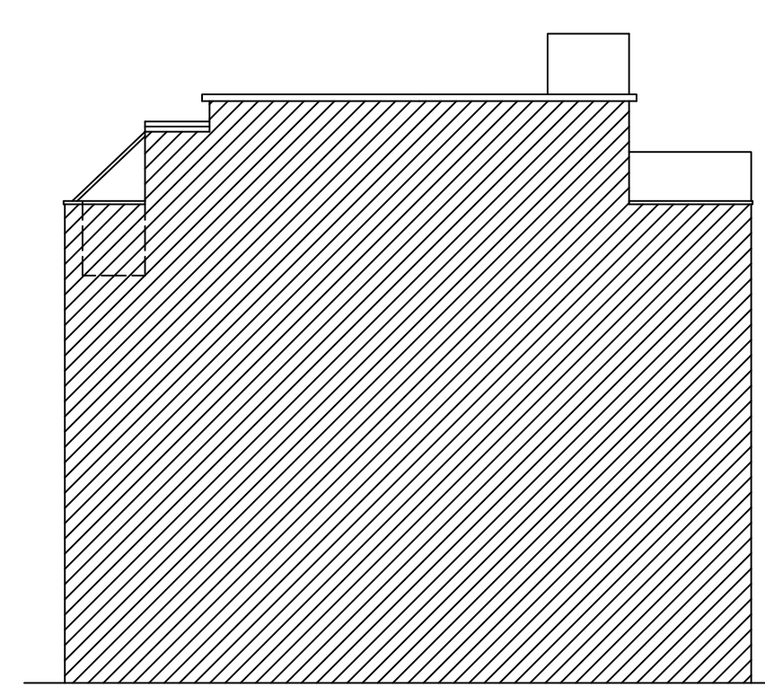
EXISTING ADJ. SIDE ELEVATION (scale 1:100)
