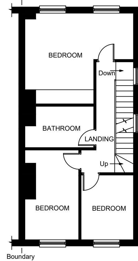
EXISTING FIRST FLOOR PLAN (scale 1:100)
