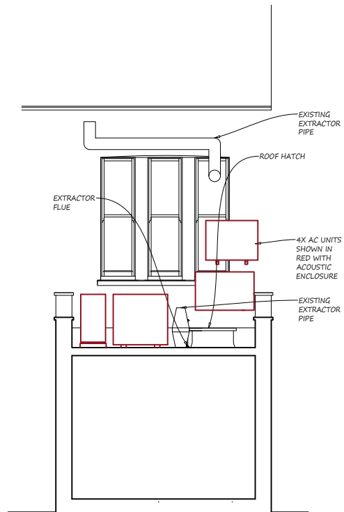
PROPOSED SECTION B-B 1:100
