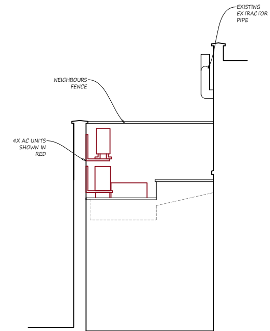
EXISTING SIDE ELEVATION 1:100
