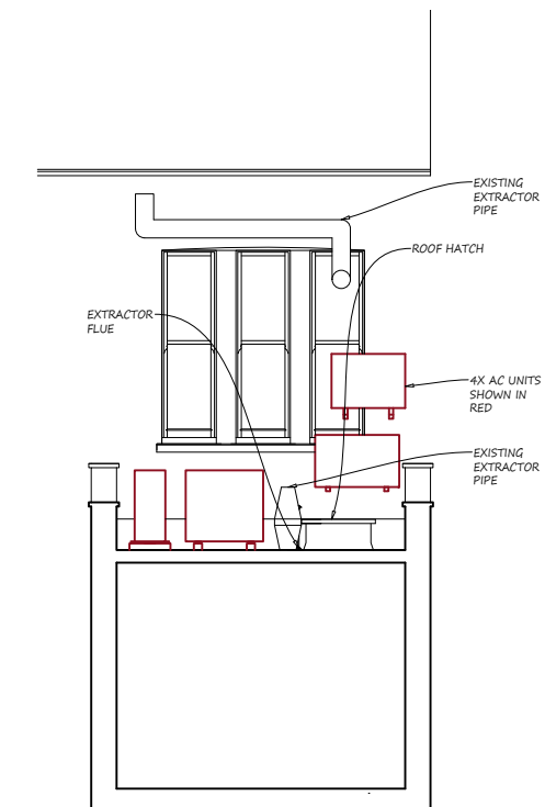
EXISTING SECTION B-B 1:100
