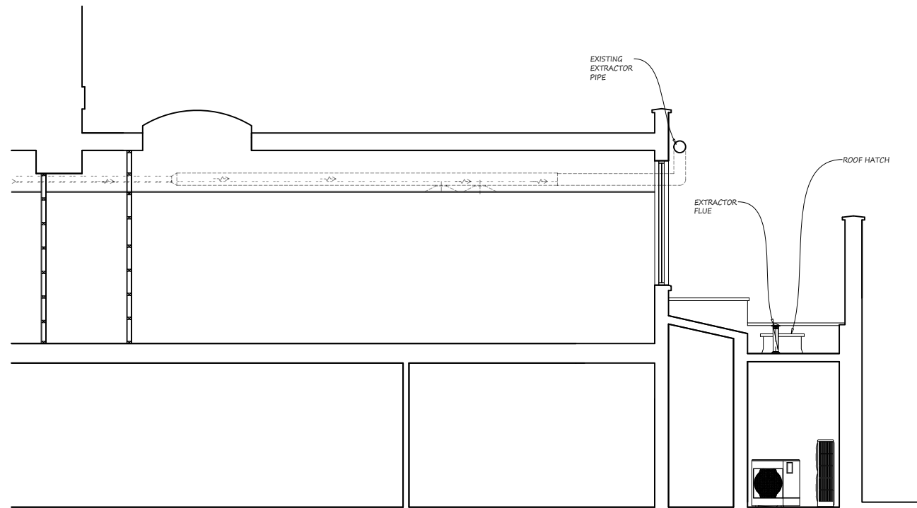
PRE-EXISTING SECTION A-A 1:100
