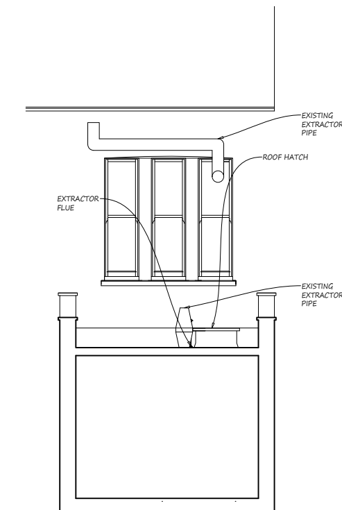
PRE-EXISTING SECTION B-B 1:100
