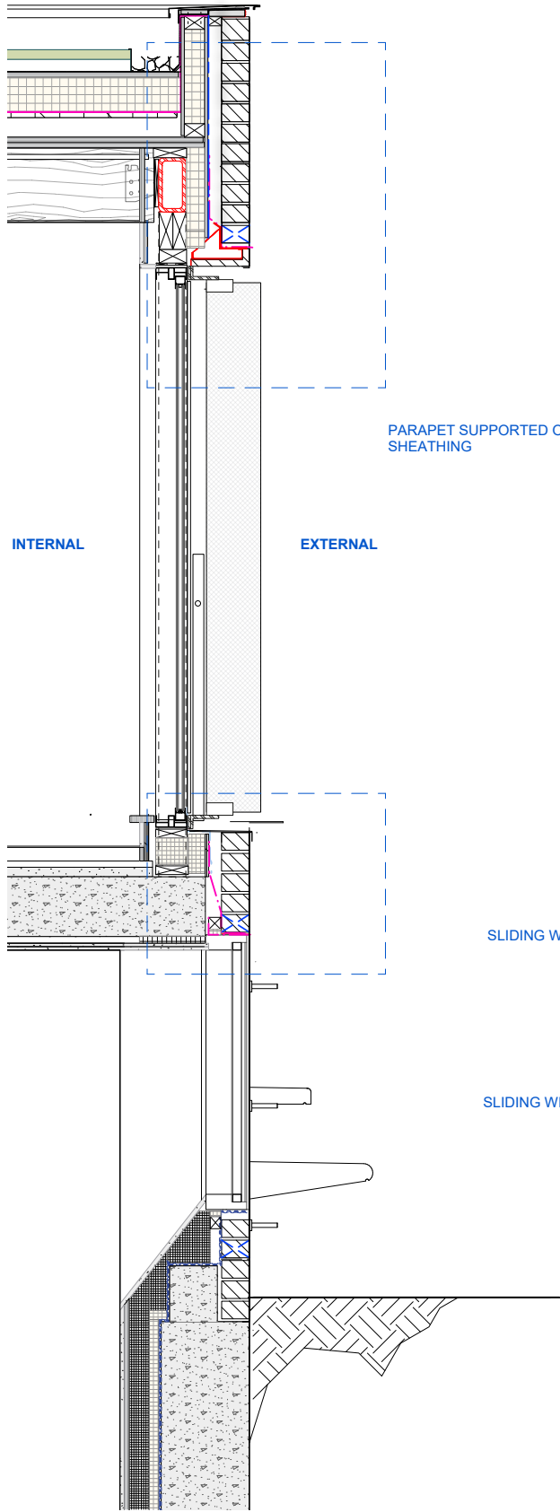
1 South Facade Details (1 of 2)
