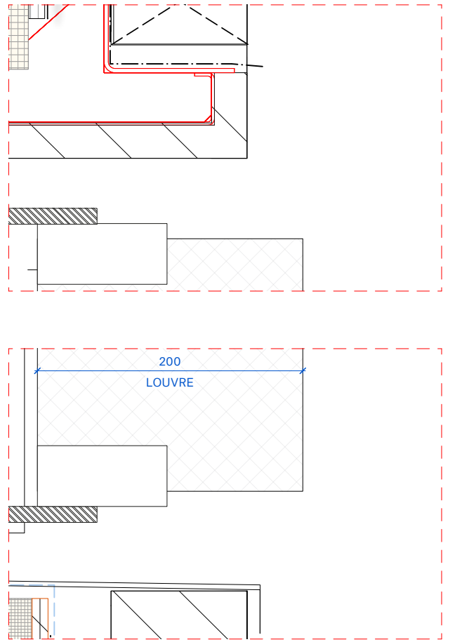
4 South Facade Details (1 of 2)
