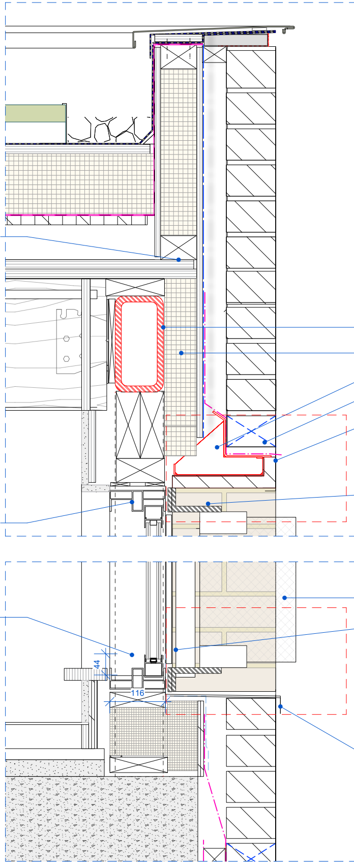
2 South Facade Details (1 of 2)
