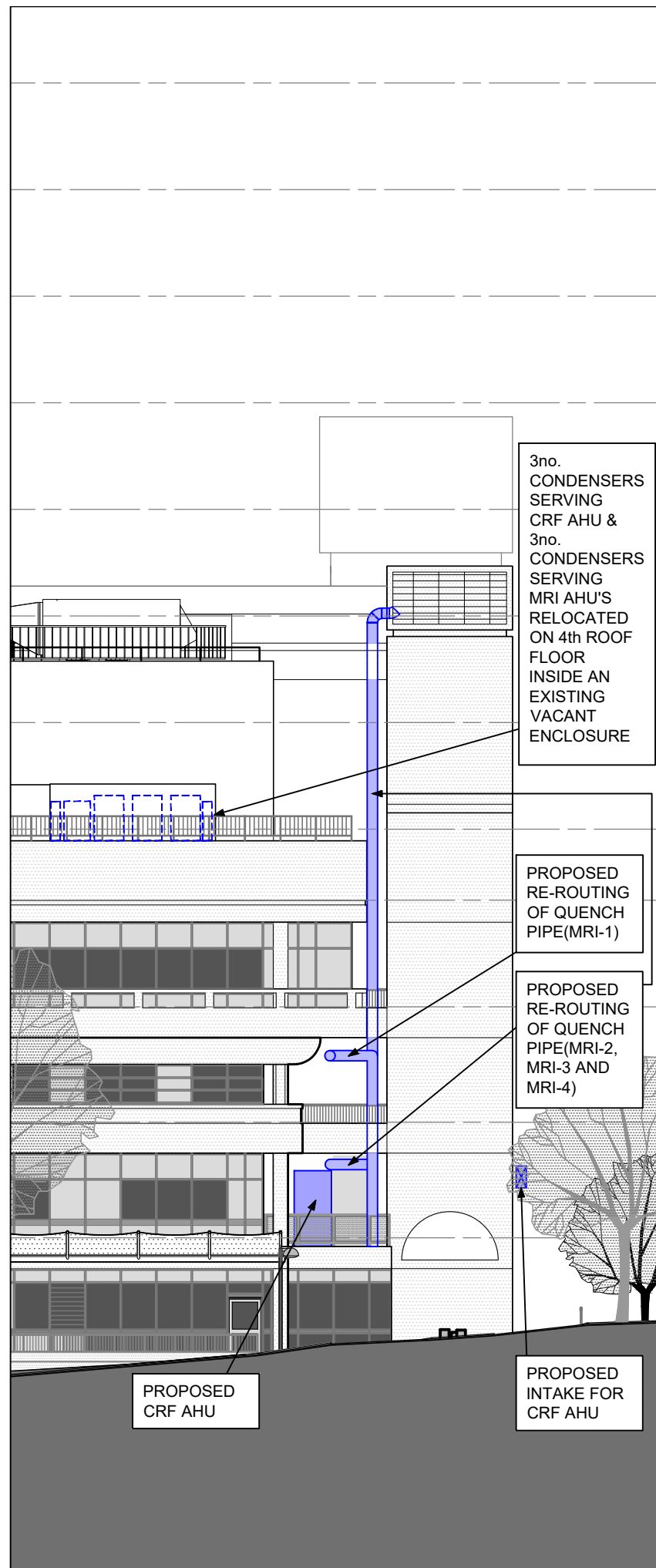
02 Proposed North Elevation - Permanent works (02)011 1:200 @ A3
