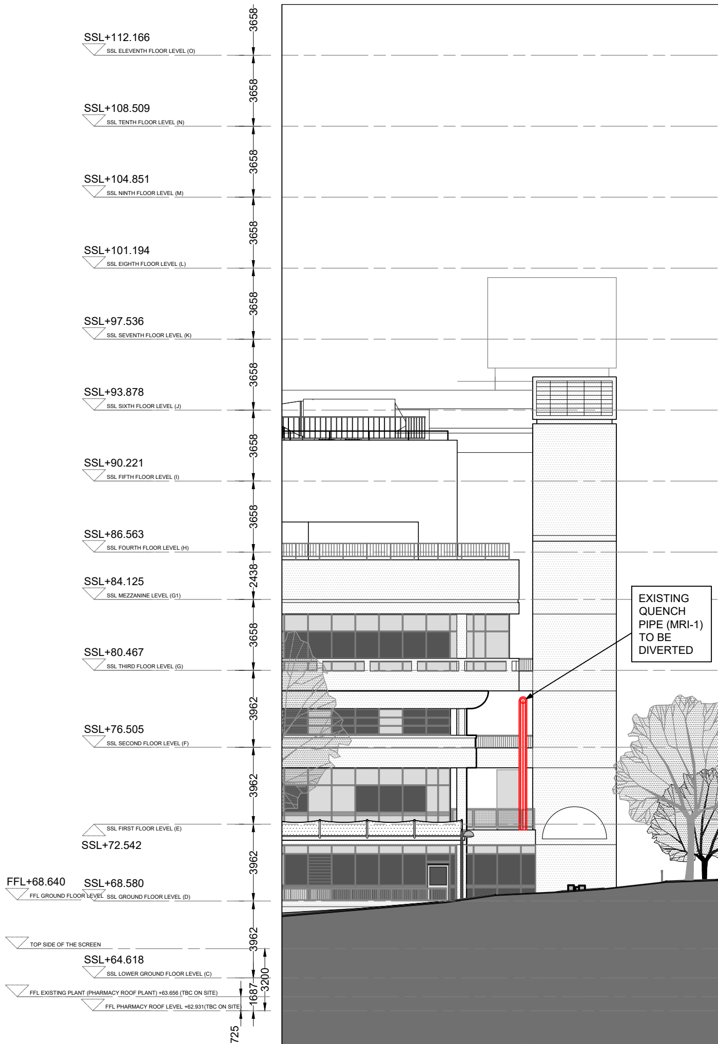
01 Existing North Elevation - Permanent works (02)011 1:200 @ A3
