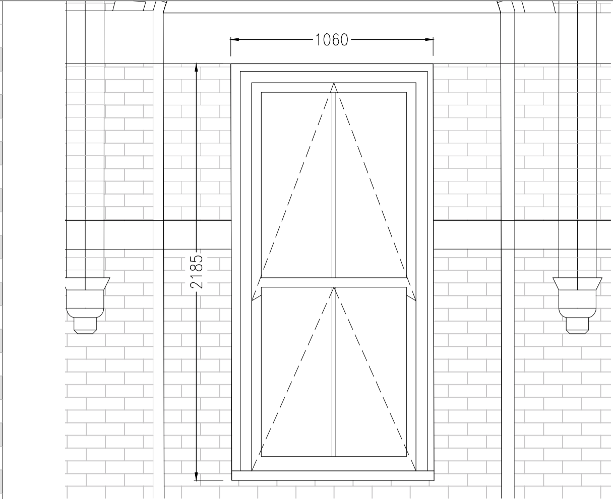
WINDOW TYPE 'A' 1:20
