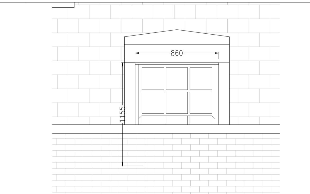
WINDOW TYPE 'F' 1:20
