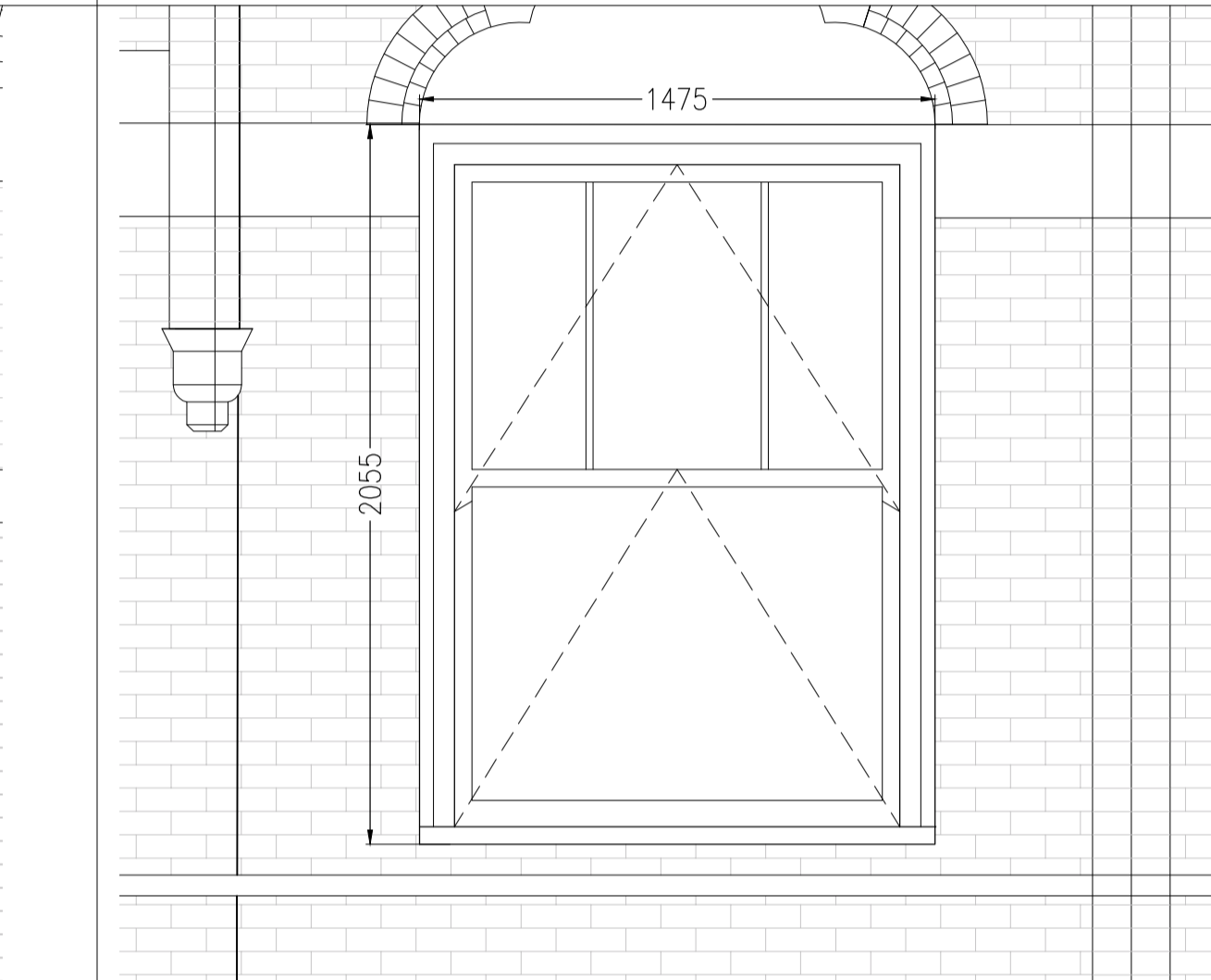
WINDOW TYPE 'D' 1:20
