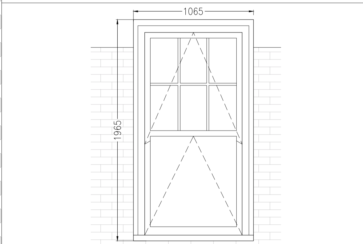
WINDOW TYPE 'E' 1:20
