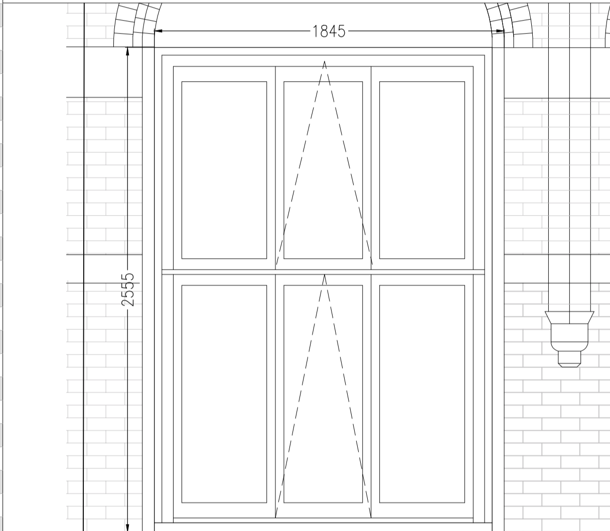
WINDOW TYPE 'C' 1:20
