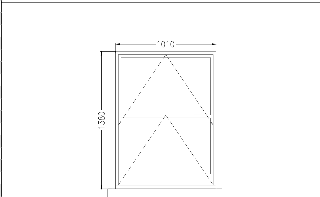
WINDOW TYPE 'E' 1:20
