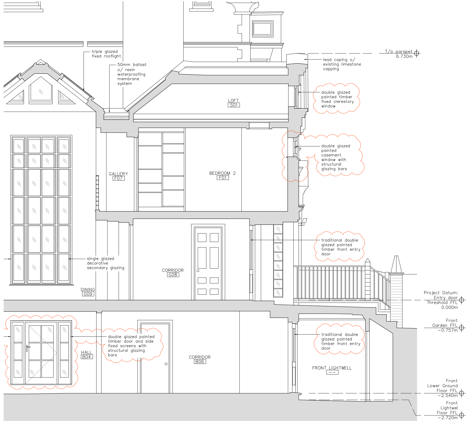
PROPOSED BUILDING SECTION AA' (SOUTH)
