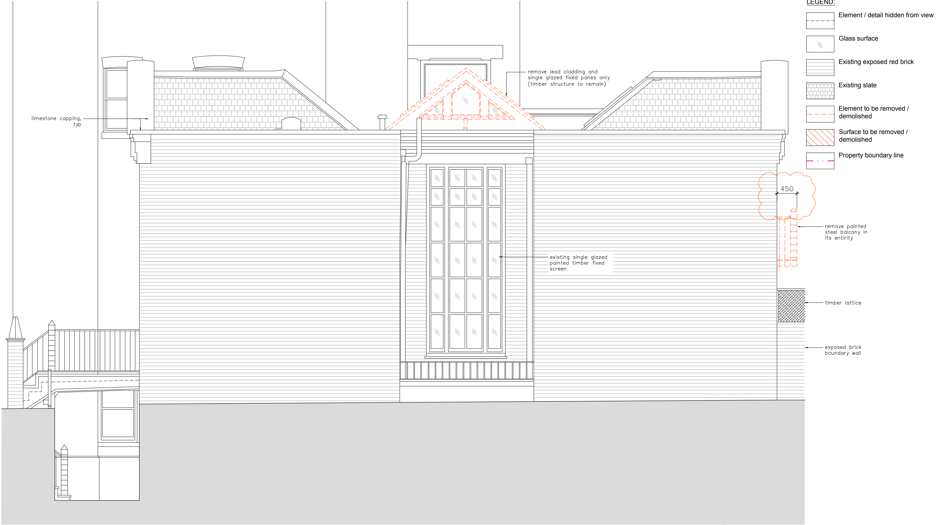
EXISTING SIDE ELEVATION EAST 1
