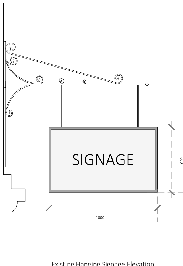
Existing Hanging Signage Elevation 1:20
