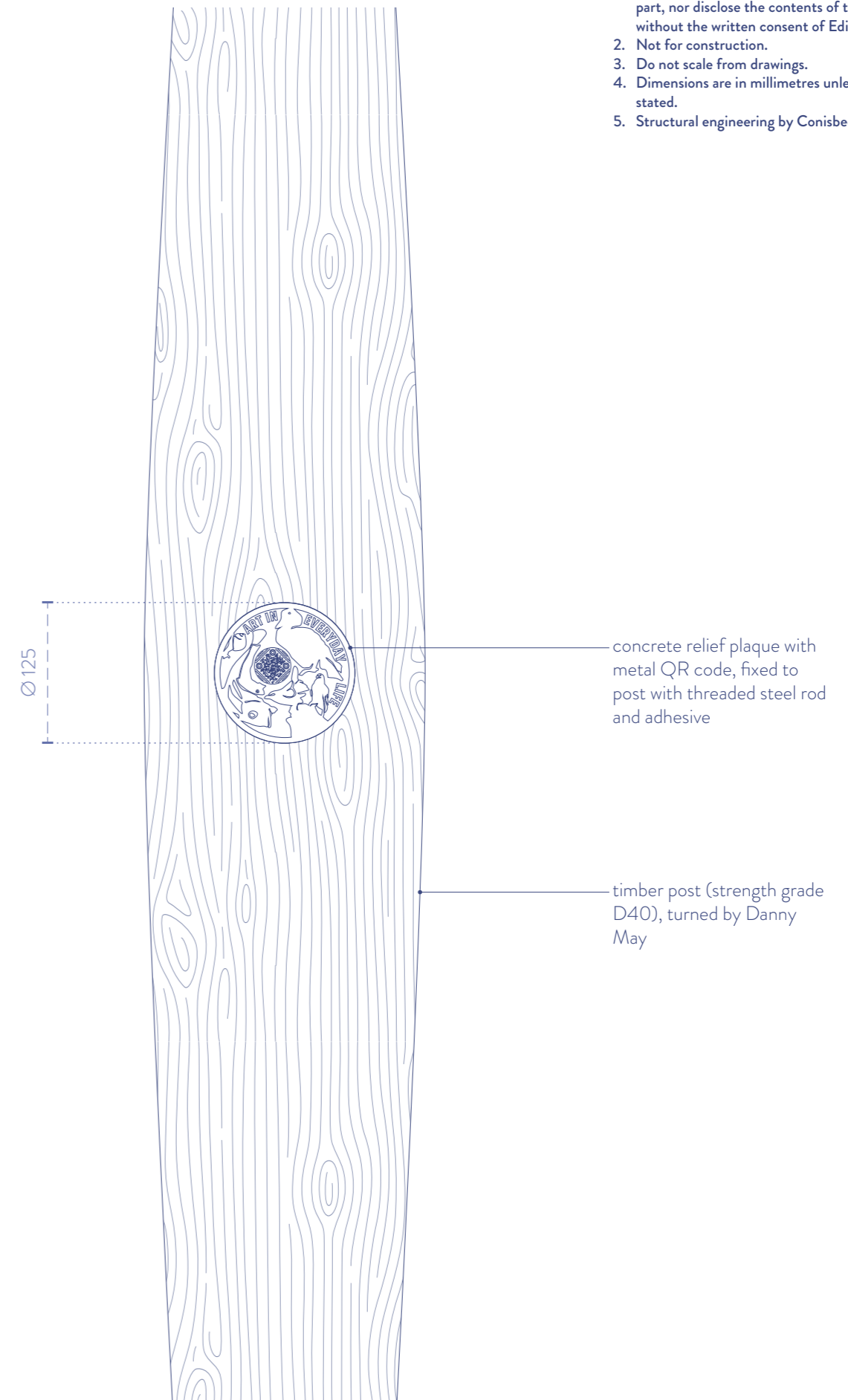
Pavement elevation
