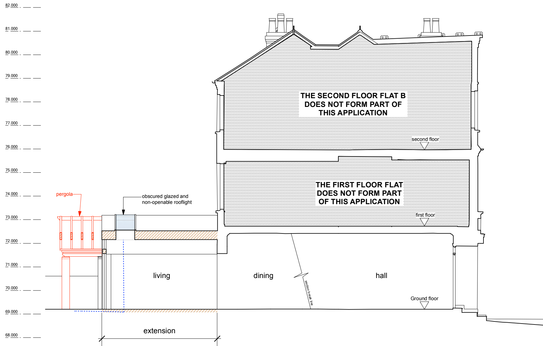
PROPOSED SECTION A-A
