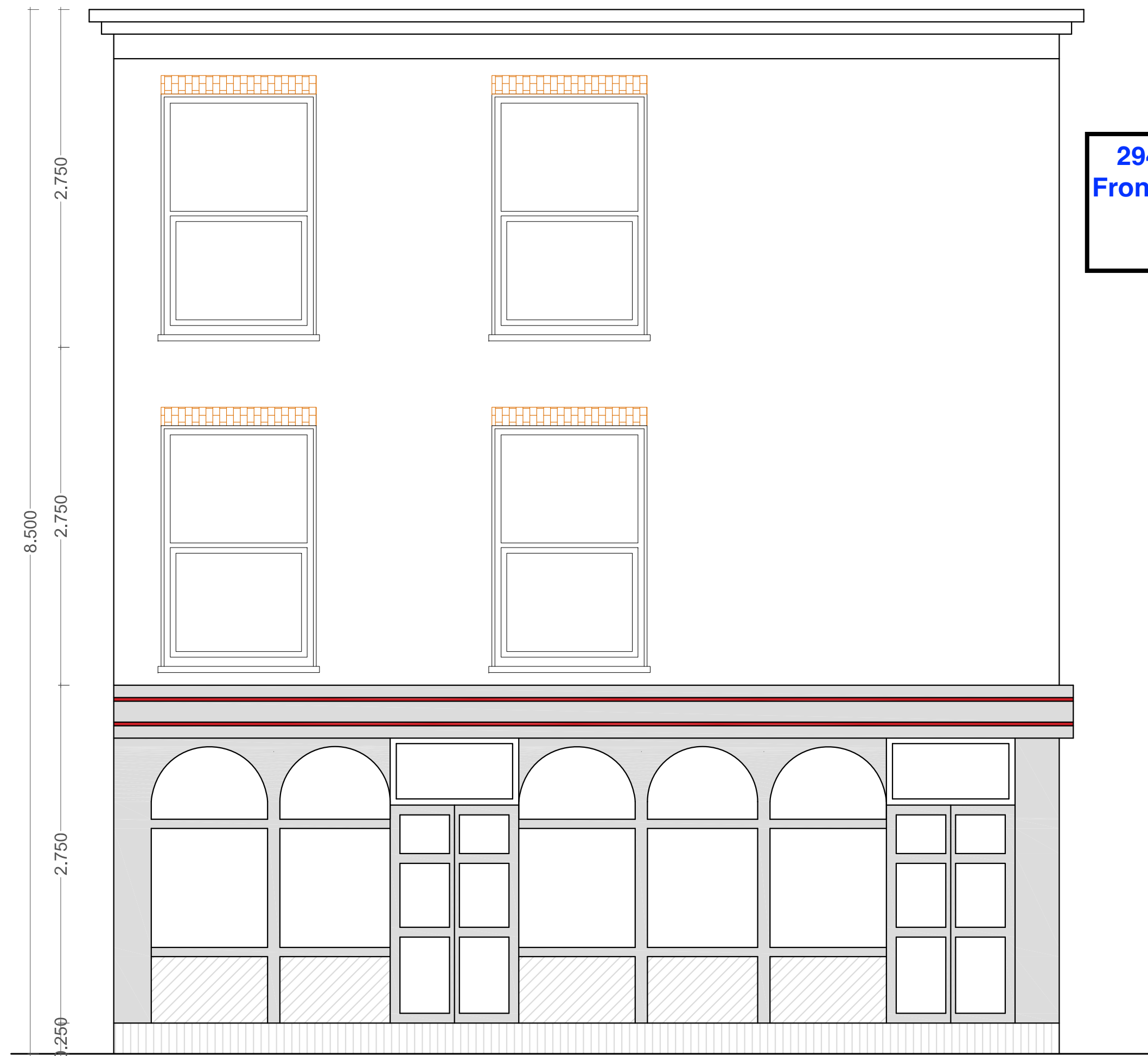
FRONT ELEVATION (Existing)
