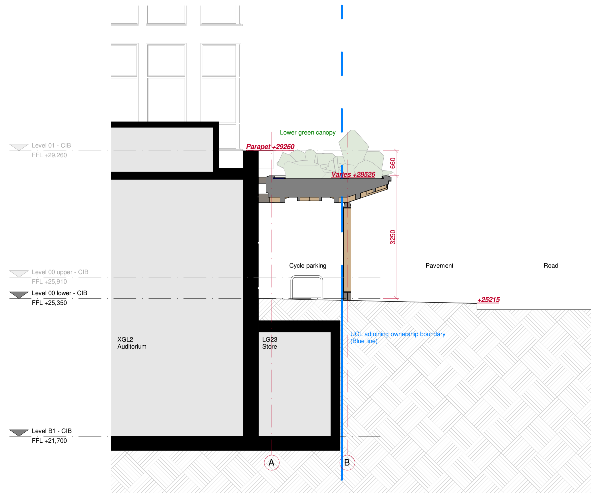
A Section A - Through lecture theatre Scale 1 : 50
