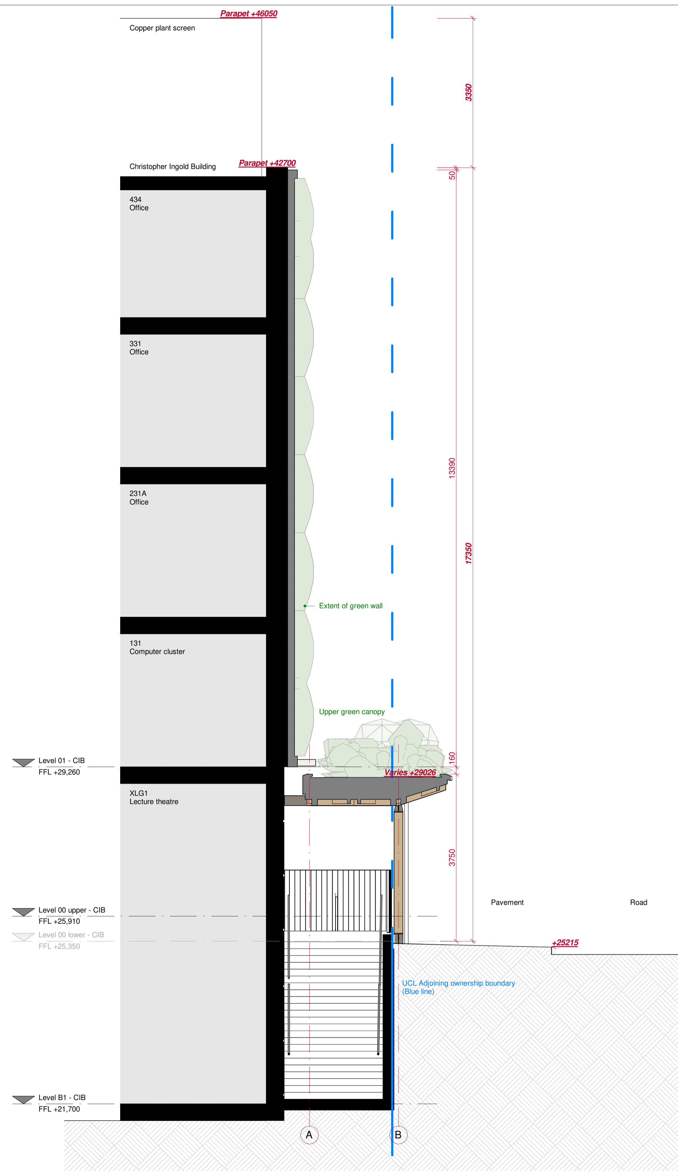
B Section B - Through escape stair Scale 1 : 50
