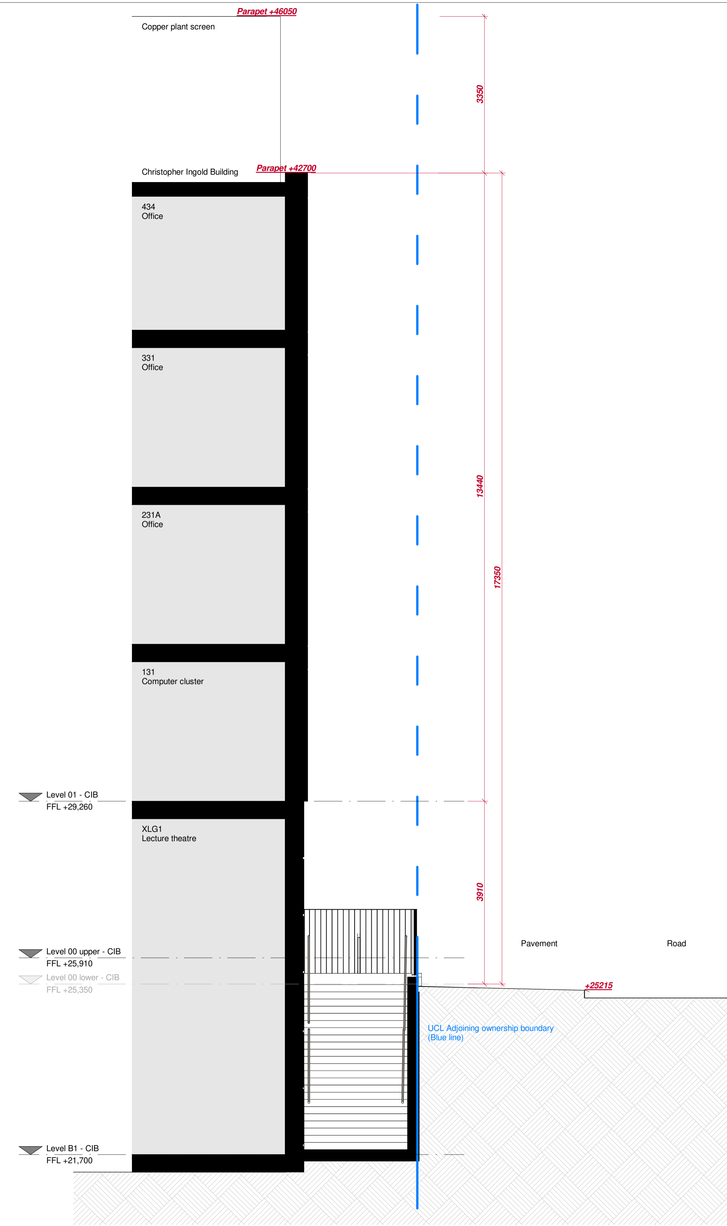
B Section B - Through escape stair Scale 1 : 50
