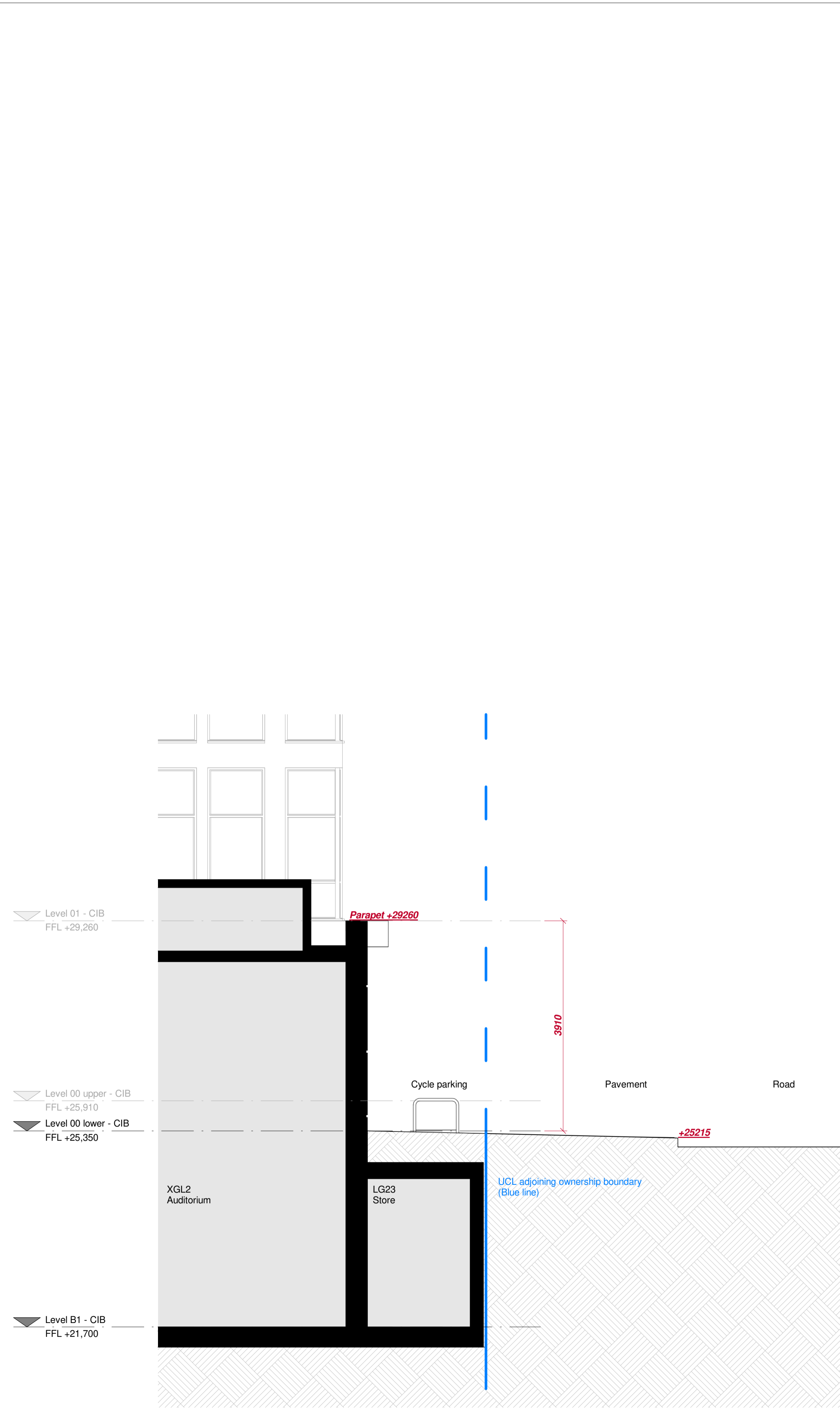
A Section A - Through lecture theatre Scale 1 : 50
