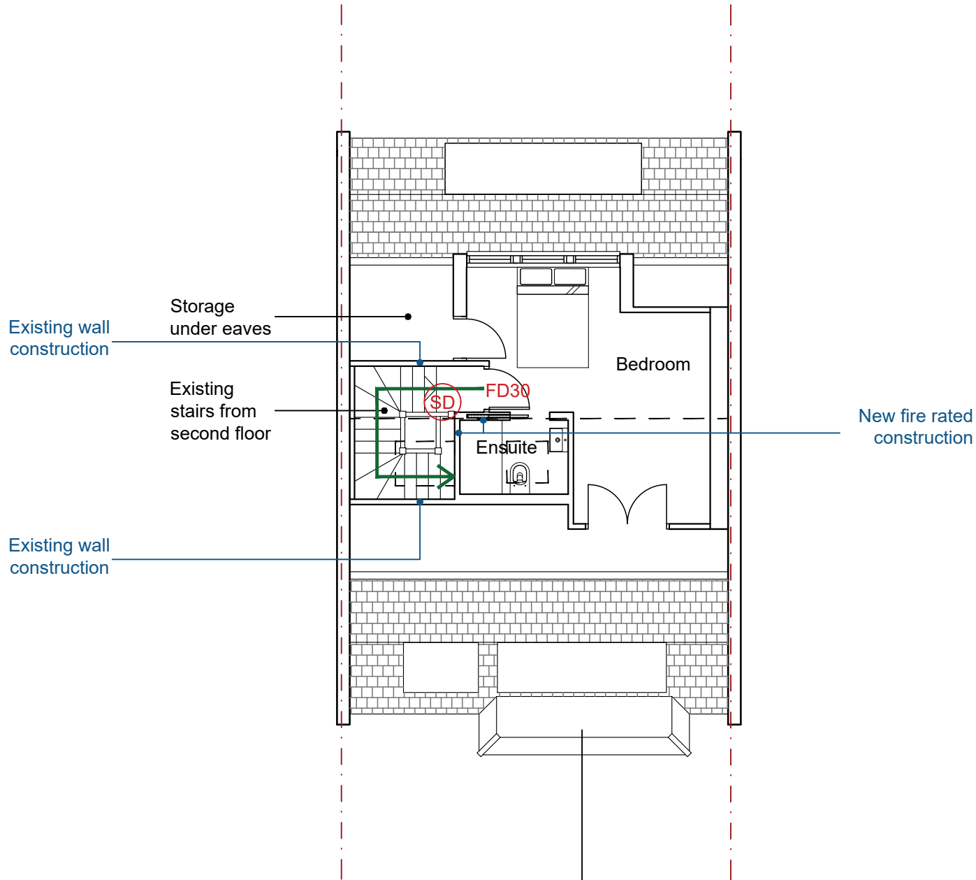
1 Proposed Third Floor Plan 1:100
