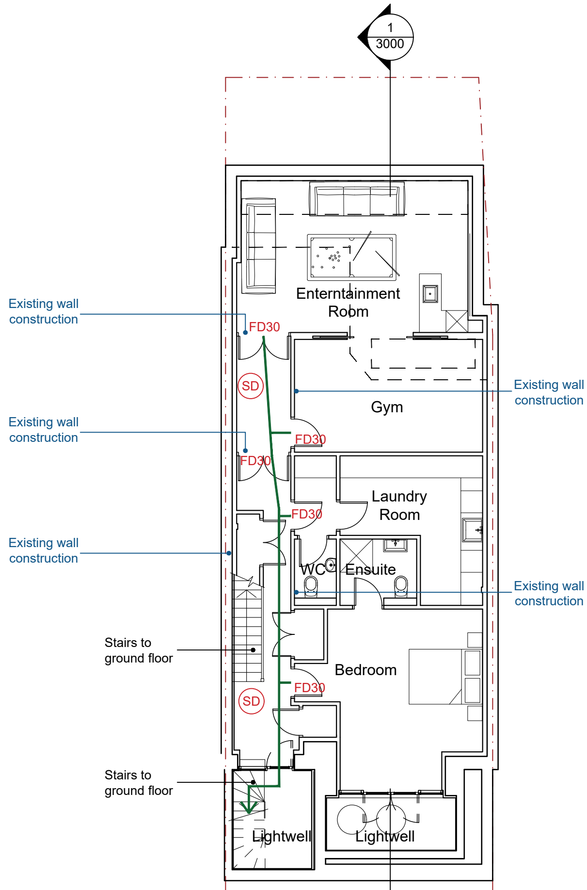
1 Proposed Basement Plan - NO CHANGES TO LAYOUT 1:100
