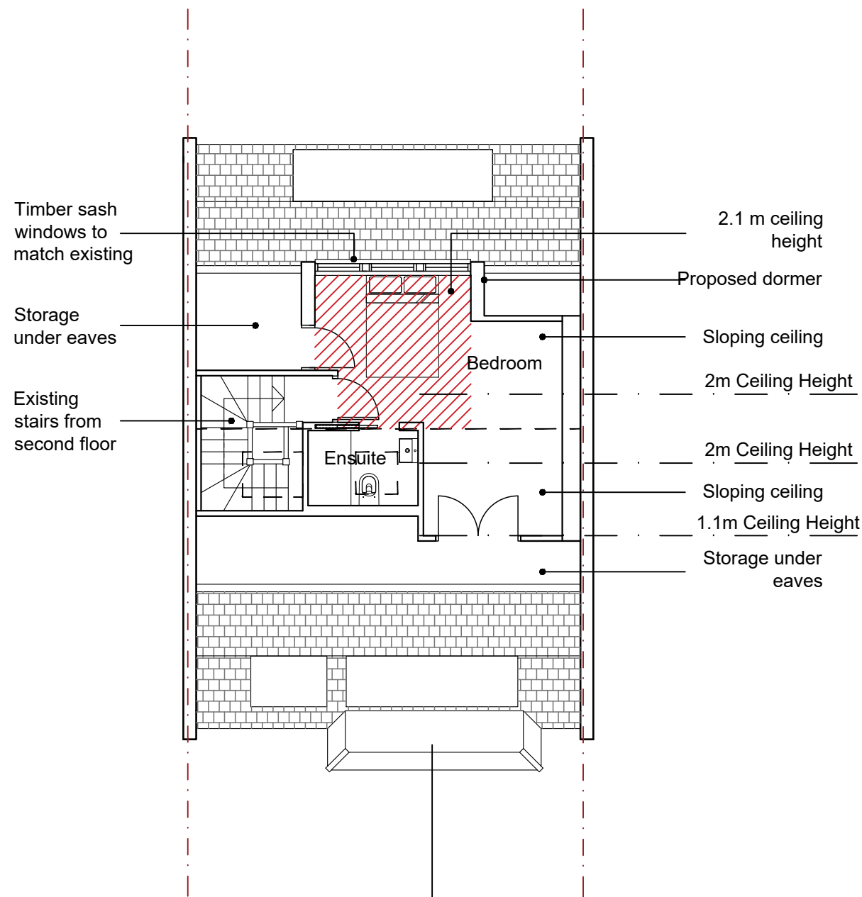
Proposed Third Floor Plan 1:100
